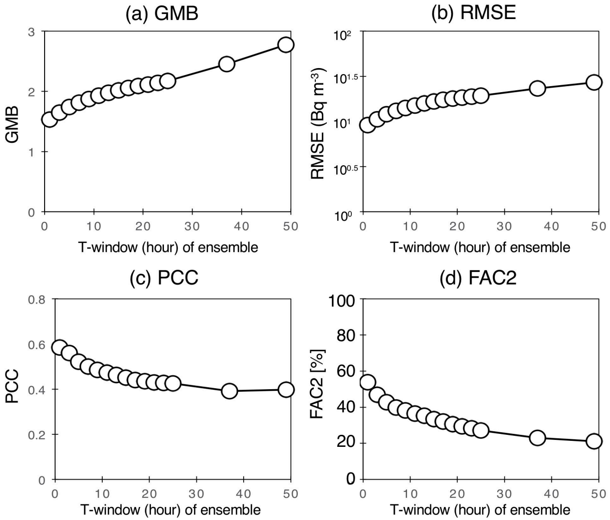
Figure 9: Statistical metrics (GMB, RMSE, PCC and FAC2) at the 101 available sites against various time windows (X-axis) ranging from 1 hour to 49 hours.
