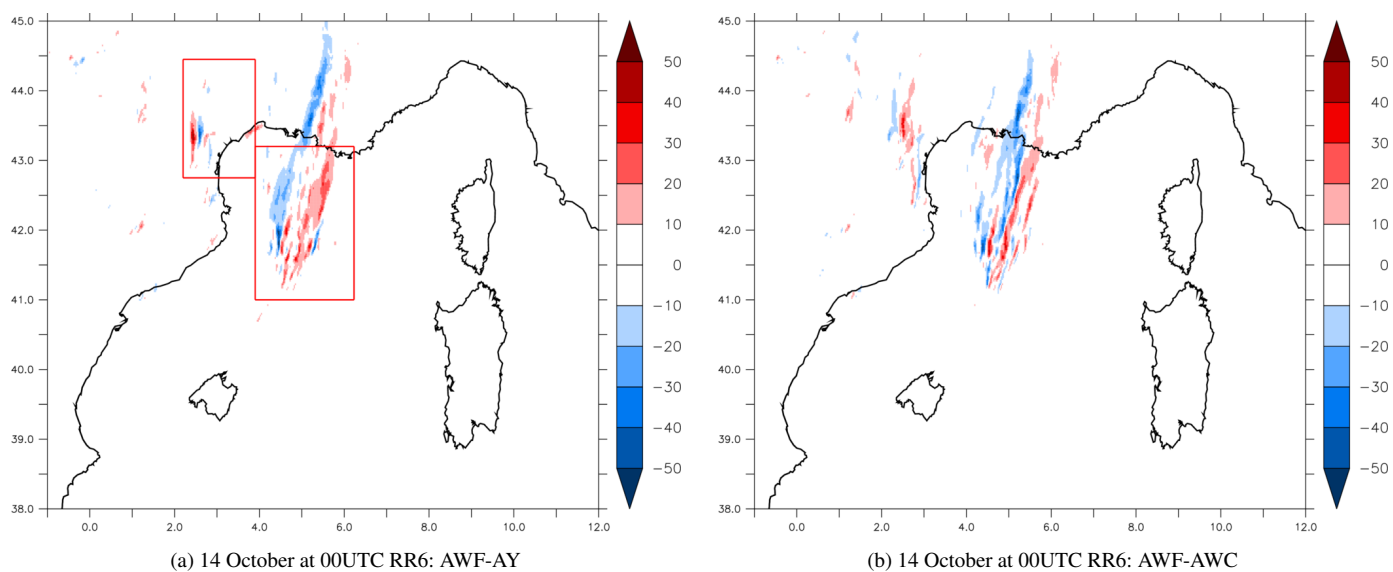
Figure 12. 6h-rainfall amount (mm) differences for the 14 October at 00UTC between AWF-AY (a) and AWF-AWC (b).
