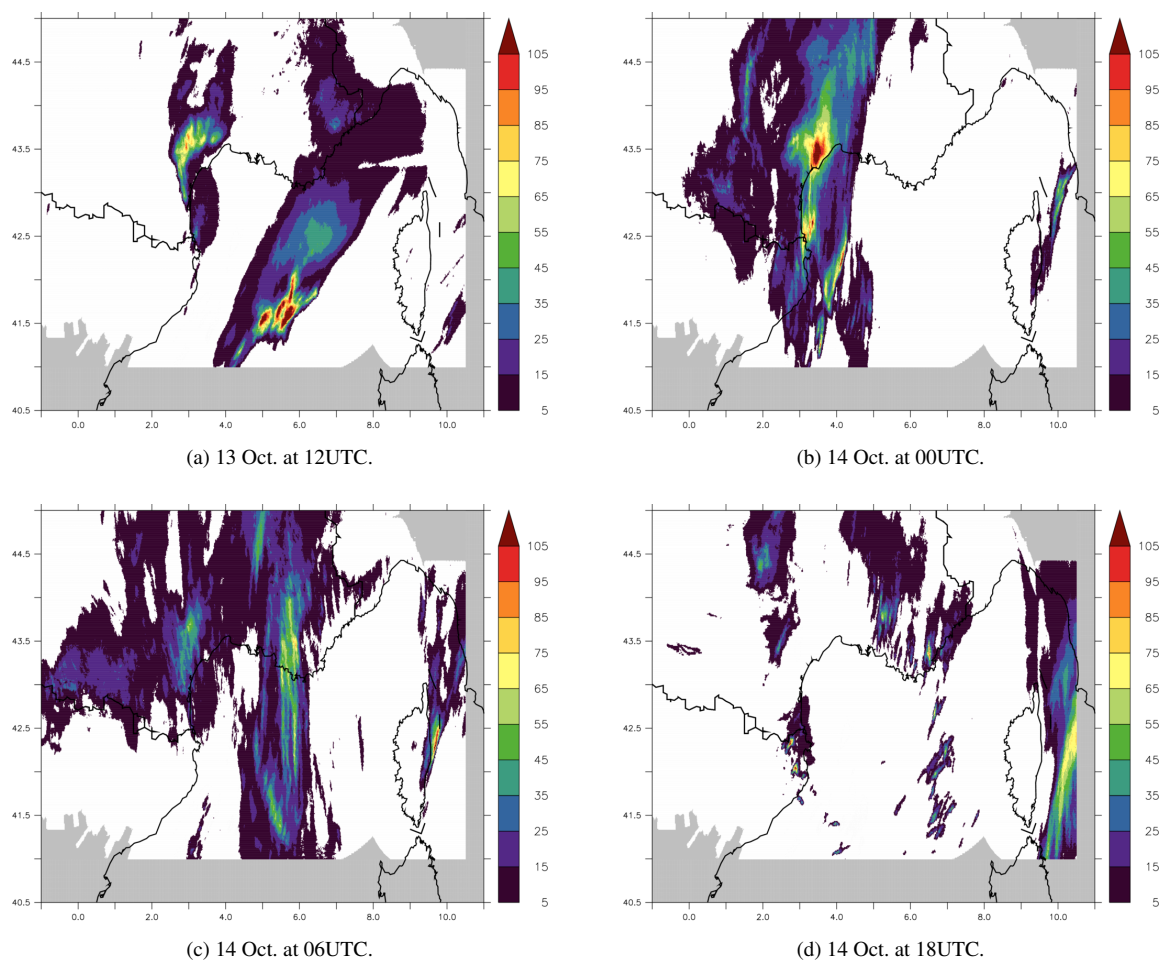
Figure 4. 6h-rainfall amounts (mm) from ANTILOPE observations.
