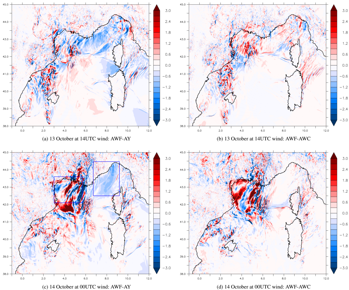
Figure 10. Wind (m.s -1 ) differences for the 13 October at 14UTC (a,b) and the 14 October at 00UTC (c,d) between AWF-AY (a,c) and AWF-AWC (b,d).
