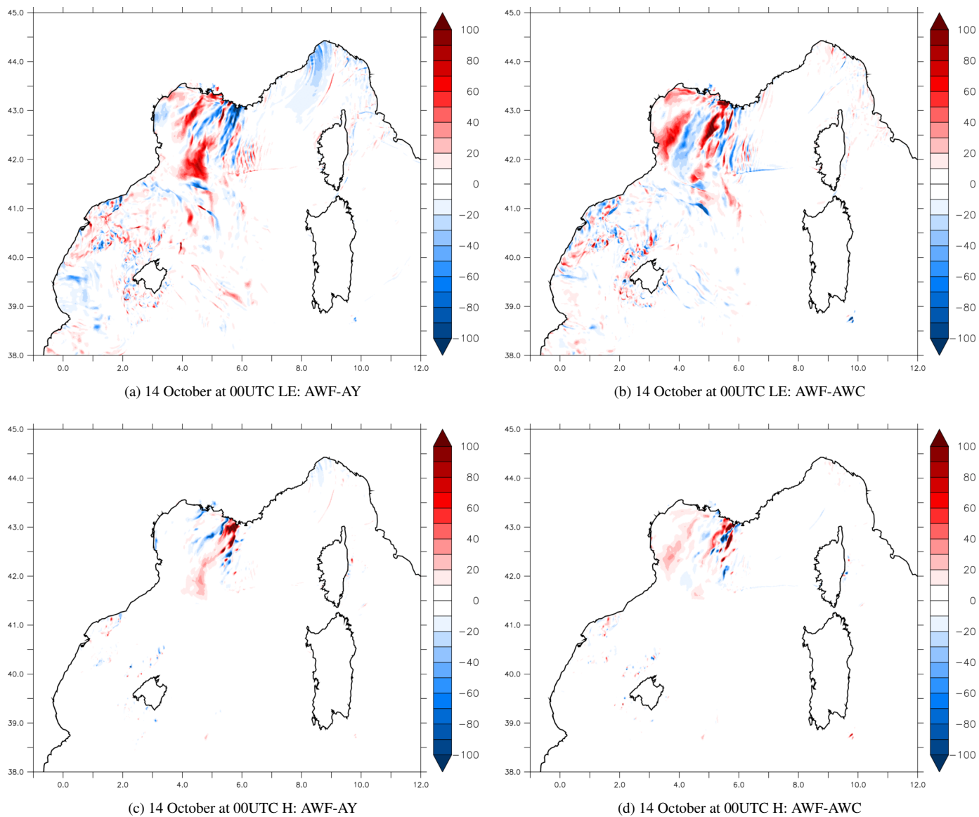
Figure 11. (a,b) LE ( \text{W.m}^{-2} ) and (c,d) H ( \text{W.m}^{-2} ) differences for the 14 October at 00UTC between AWF-AY (a,c) and AWF-AWC (b,d).
