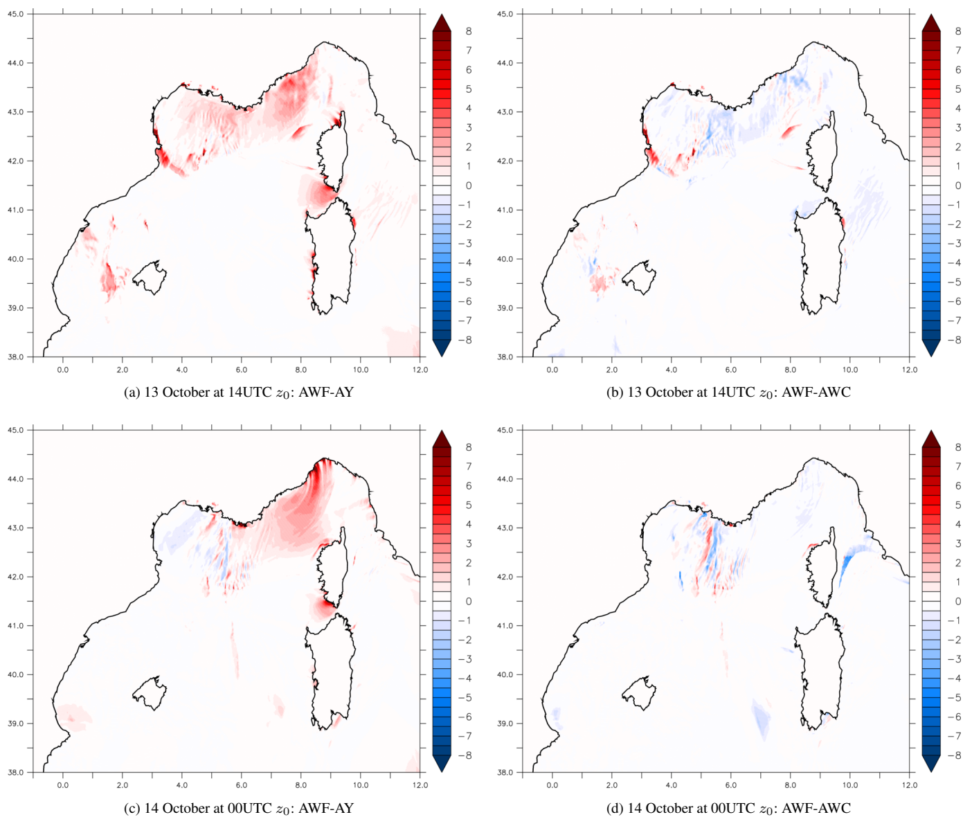
Figure 9. z_0 ( 10^{-3} m) differences for the 13 October at 14UTC (a,b) and the 14 October at 00UTC (c,d) between AWF-AY (a,c) and AWF-AWC (b,d).
