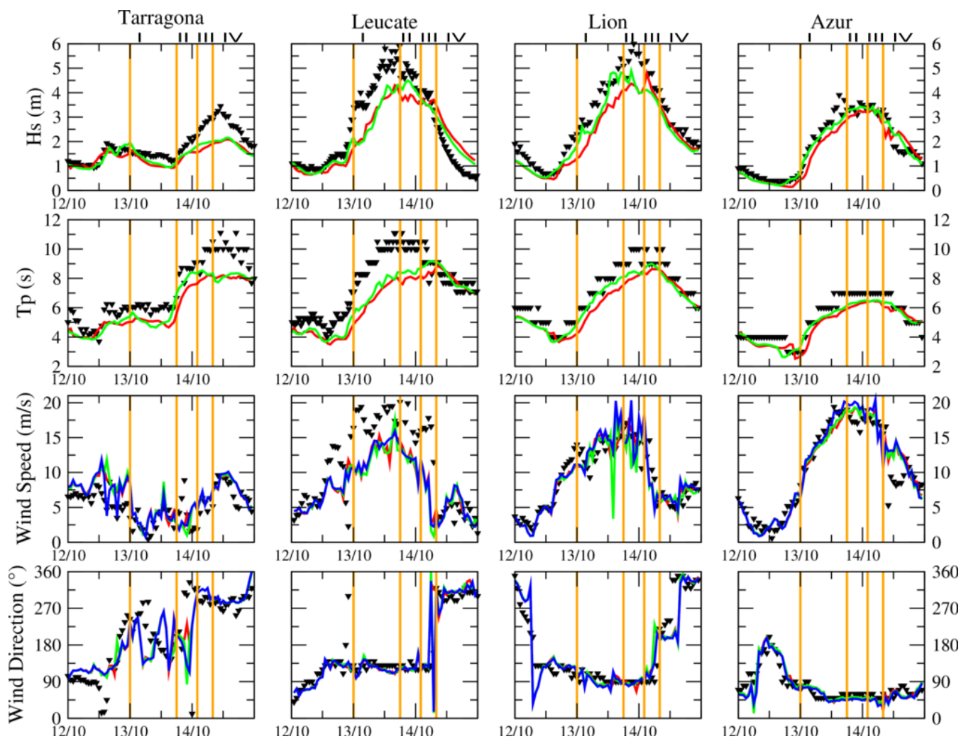
Figure 2. Evolution of H_s (m), T_p (s), wind speed ( \text{m}\cdot\text{s}^{-1} ) and wind direction ( ^\circ ) simulated with AWF (green for atmospheric parameters), AWC (red), AY (blue) and WY (green for wave parameters) against buoy observations (black triangles).
