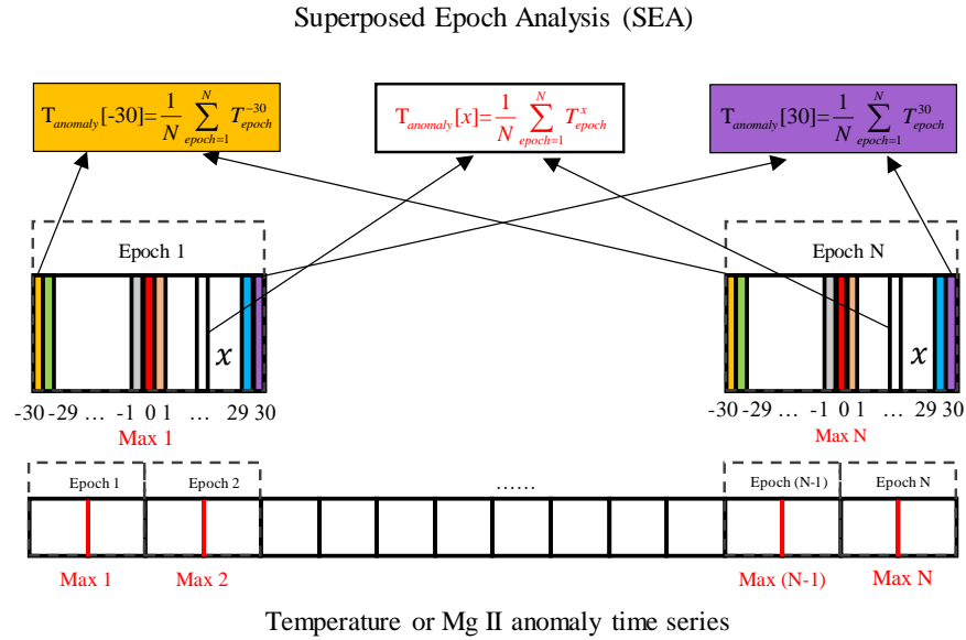
Figure 5. Overview of the superposed epoch analysis (SEA). It should be noted that the epochs are allowed to overlap even we do not show it on the figure.
