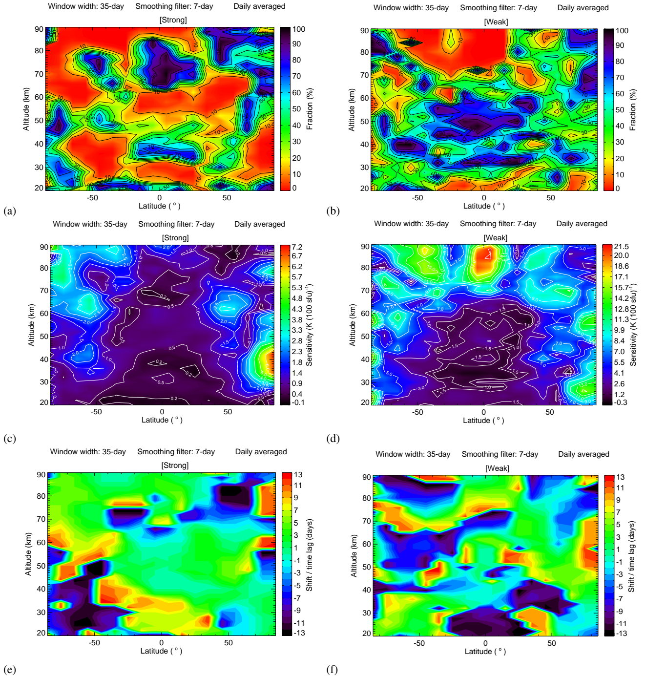
Figure 12. (a–b) Similar to Figure 9 (a), except for strong and weak solar activity years. (c–f) Sensitivity and shift for the latitude from 85^{\circ} S to 85^{\circ} N and the altitude from 20 to 90 km for different solar activity.
