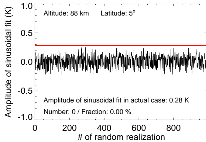
Figure 8. Illustration of the Monte-Carlo significance test for an altitude of 88 km and a latitude of 5° N. The red line shows the amplitude of a sinusoidal fit to the extracted 27-day signatures in MLS daily averaged temperature. The black line shows the fitted amplitudes to epoch-averaged temperature anomalies for 1000 randomly chosen epoch ensembles.
