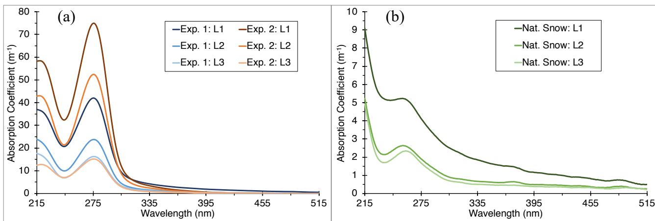
5 Figure 4. Absorption coefficient of snow meltwater for layers L1, L2, and L3 for deposited BrC (Panel a) and for background impurities occurring in the natural snowpack (Panel b). “Exp. 1” and “Exp. 2” refer to the first and second BrC deposition experiments, respectively. The spectra of the natural snow (Panel b) have been averaged for two locations at the experiment site.
