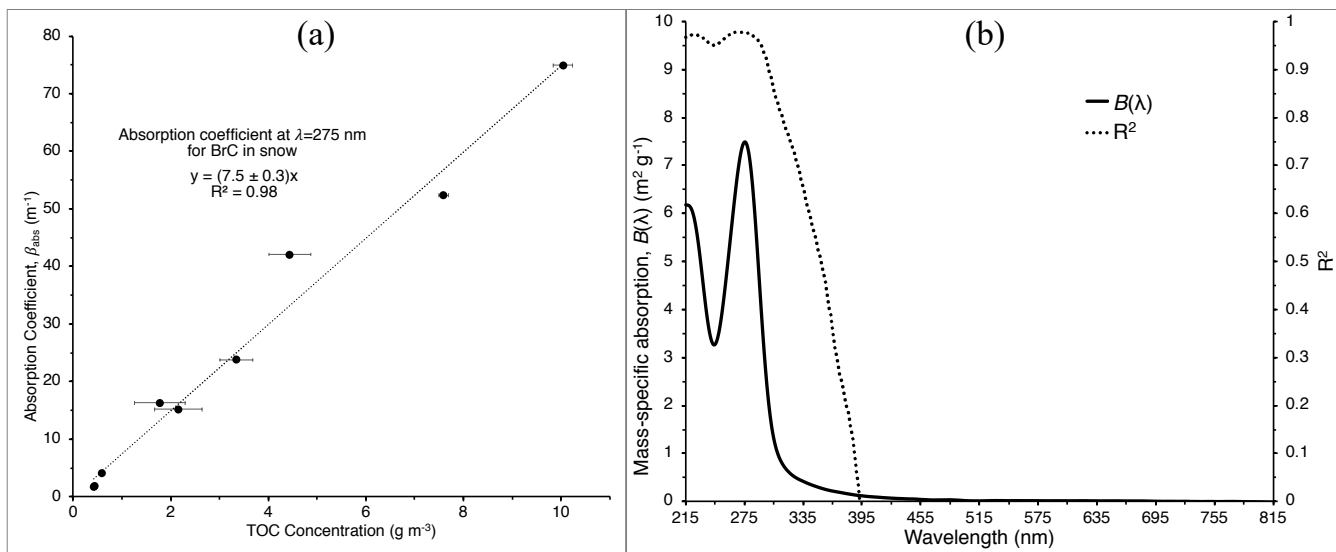
10 Figure 5. Panel (a): Absorption coefficient at 275 nm as function of total organic carbon (TOC) concentration. The fitted linear regression slope gives the mass-specific absorption B_{\lambda} = 7.5 \pm 0.3 \text{ m}^2 \text{ g}^{-1} with a correlation coefficient of R^2 = 0.98 . Panel (b): Mass-specific absorption, B(\lambda) , and R^2 for each value of B(\lambda) across the wavelength range 215 – 815 nm for BrC deposited experimentally and found in natural snow at Tamarack Lake together at a 1-nm resolution. These panels include absorption coefficients of all meltwater samples characterized in Fig. 2.
