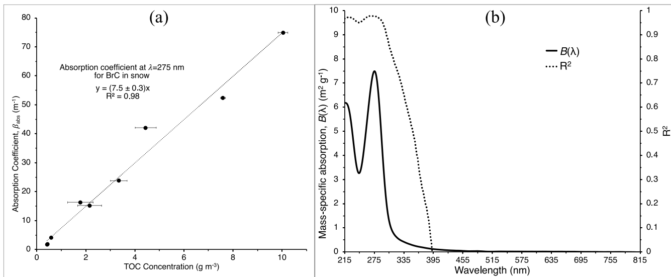
5 Figure 5. Panel (a): Absorption coefficient at 275 nm as function of total organic carbon (TOC) concentration. The fitted linear regression slope gives the mass-specific absorption B_{\lambda} = 7.5 \pm 0.3 \text{ m}^2 \text{ g}^{-1} with a correlation coefficient of R^2 = 0.98 . Panel (b): Mass-specific absorption, B(\lambda) , and R^2 for each value of B(\lambda) across the wavelength range 215 – 815 nm for BrC deposited experimentally and found in natural snow at Tamarack Lake together- at a 1-nm resolution . These panels include absorption coefficients of all meltwater samples characterized in Fig. 2.
