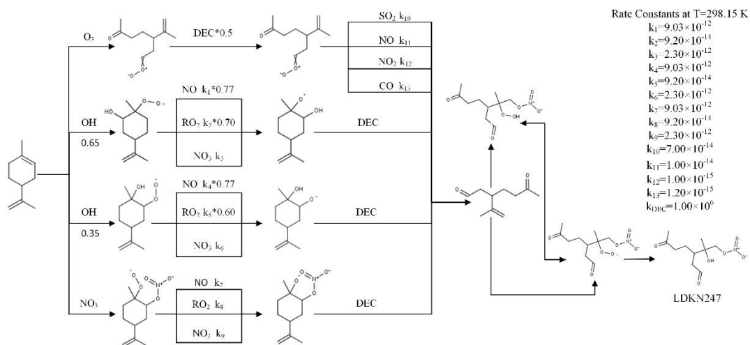
Figure S1. Formation mechanism of LDKN247 from limonene in the Master Chemical Mechanism (MCM).
