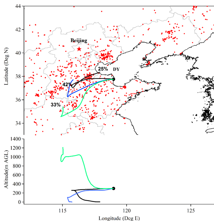
Figure S2. Distribution of fires and 48-h backward trajectories on 15 June, 2017 at DY site.
