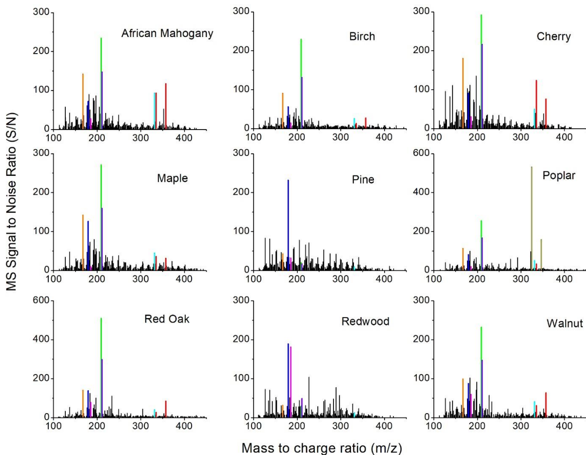
Figure 3: High resolution mass spectra of WSA extracts in the study, taken at 100 \mu\text{g/mL} concentration. The color key for highlighted peaks with proposed assignments for the major species at each peak is: Orange – \text{C}_9\text{H}_{10}\text{O}_3 , acetovanillone or homovanillin (protonated); Blue – \text{C}_{10}\text{H}_{10}\text{O}_3 , coniferyl aldehyde (protonated); Magenta – \text{C}_6\text{H}_{10}\text{O}_5 , levoglucosan, mannosan, or galactosan (sodiated); Green – \text{C}_{11}\text{H}_{12}\text{O}_4 , sinapaldehyde (protonated); Cyan – \text{C}_{18}\text{H}_{18}\text{O}_6 , G-vanillin dimer (protonated); Red – \text{C}_{18}\text{H}_{22}\text{O}_6 , various S-G dimers (protonated and sodiated); Dark yellow – \text{C}_{20}\text{H}_{21}\text{NO}_3 , unknown alkaloid (protonated and sodiated)..
