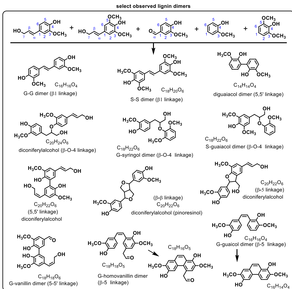
Figure 4: Proposed chemical structures of some monomers and dimers observed in this work. More than one structure may be present at each molecular formula.
