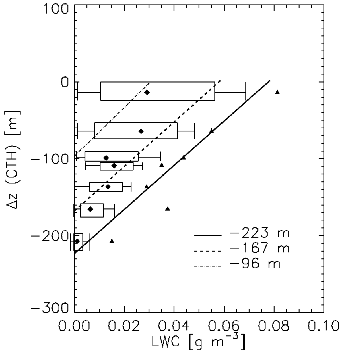
Figure 8. LWC profile percentiles relative to CTH for the mixed-phase cloud layer with data from Nevzorov LWC sensor. Theoretical adiabatic ascents are shown, starting from three altitudes (see legend for details) which correspond to potential cloud bases (see text for details). Statistics as Fig. 4.
