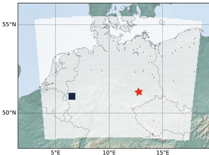
Figure 1. Model domain over Germany, which was used in this study (white area). The red star marks the research station Melpitz (12.93°E, 51.53°N) and the blue square the measurement site Jülich (50.88°N, 6.41°E).
