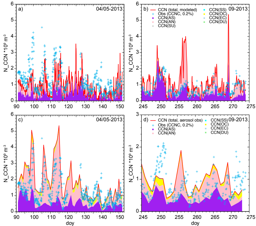
Figure 2. Simulated and measured CCN number concentrations in Melpitz at a supersaturation of 0.2 % during the two HOPE campaigns (April to May and September 2013). The upper panel (a and b) shows the CCN number concentrations resulting from the simulated aerosol concentrations, the lower one (c and d) the CCN numbers resulting from measured aerosol concentrations using the same CCN parametrization. The colors represent the contributions to CCN of different species. The blue crosses indicate the CCN number concentrations using the CCNC. Please note the different time resolution for the observations, as well as the different scale for the CCN number concentration in plot d.
