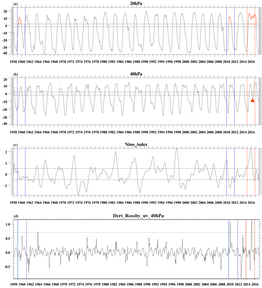
Figure 1. Zonal mean zonal wind at (a) 20 hPa, (b) 40 hPa, (c) ENSO index in the Niño 3.4 region. Panel (d) denotes the time series of the horizontal Rossby wave momentum flux anomaly with respect to the monthly climatology averaged over the tropics (from 10°S to 10°N) at 40 hPa from 1958 to 2017 (unit is m^2/s^2 ). The horizontal dashed lines denote the speed of 2 m/s and -2 m/s in panels (a) and (b). In panel (c) the horizontal dashed lines denote 0.5 K and -0.5 K, respectively. The horizontal dashed line denotes the value of 0.7 m^2/s^2 in panel (d). The vertical red lines denote the time period of 2015/2016 and the vertical blue lines denote the periods of 1959/1960 and 2010/2011. In panel (a) the horizontal red lines denote the westerly phase periods during 1959/1960, 2010/2011 and 2015/2016 at 20 hPa. In panel (b) the red triangle denotes the reversed westerly zonal wind in 2015/2016 at 40 hPa.
