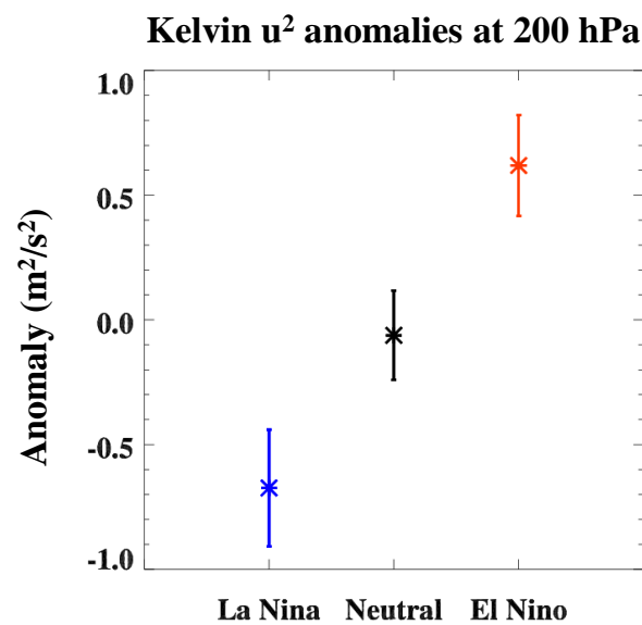
Figure 15. The squared perturbations in zonal mean zonal wind for Kelvin waves averaged over 10^\circ\text{S} - 10^\circ\text{N} at 200 hPa for La Niña (blue star), Neutral (black star) and El Niño (red star) conditions. The error bars denote \pm 1 standard deviation of the mean values.
