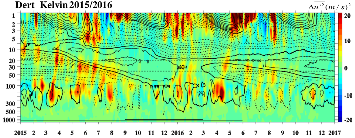
Figure 13. Temporal evolution of Kelvin wave activity as squared zonal wind anomalies averaged over 10°S-10°N in the vertical direction. Color shading denotes the anomalies with respect to the monthly climatology ( 0 \text{ m}^2 \text{ s}^{-2} ). The horizontal dashed lines denote the altitudes of 20 and 40 hPa. The zonal mean zonal wind is overlaid in black contours with contour interval of 5 \text{ m/s} . The solid and dotted black contours denote westerly and easterly winds, respectively. The thick contours represent the zero wind line. The horizontal solid lines denote the El Niño (single line) and strong El Niño periods (double line) in the bottom.
