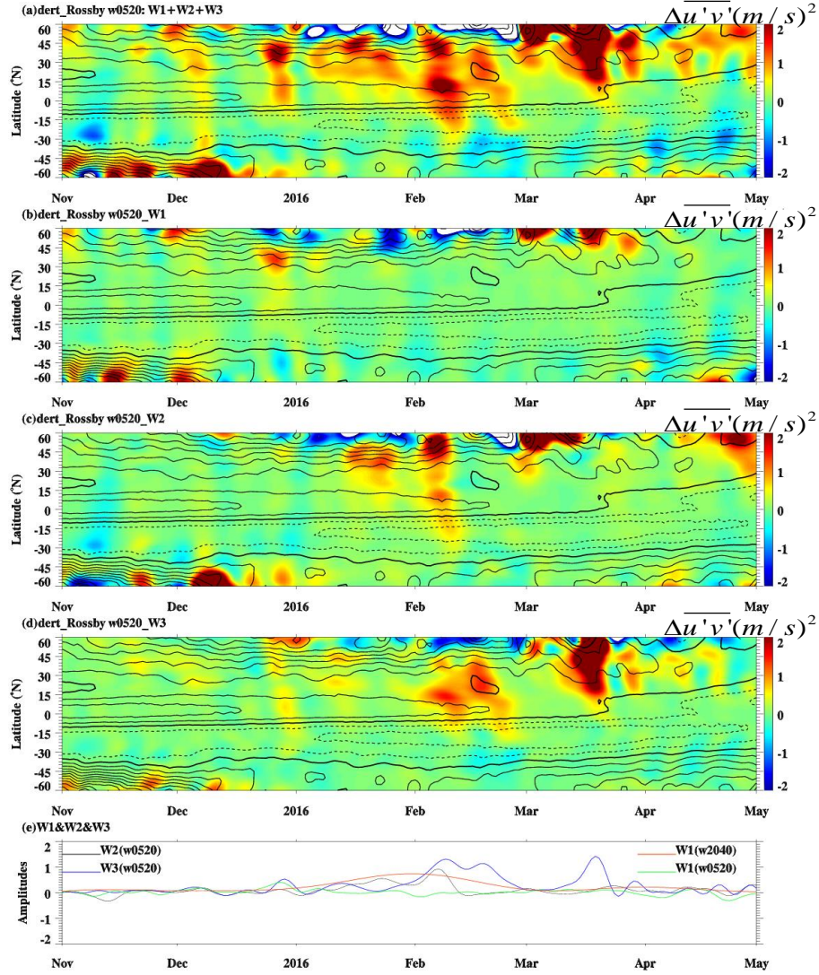
Figure 10. The time-latitude cross section of Rossby w0520 horizontal momentum flux anomalies (a) W1+W2+W3, (b) W1, (c) W2 and (d) W3 from November 2015 to April 2016. Color shadings denote the anomalies with respect to the monthly climatology ( 0 m^2 s^{-2} ). The zonal mean zonal wind is overlaid in black contours with contour interval of 5 m/s. The solid and dotted black contours denote westerly and easterly winds, respectively. The thick contours represent the zero wind line. W1, W2 and W3 denote the Rossby w0520 with wavenumber 1, 2 and 3, respectively. Panel (e) shows the horizontal momentum flux anomaly of W1, W2, W3 and Rossby w2040 (with wavenumber 1) at 40 hPa averaged from 10°N to 20°N.
