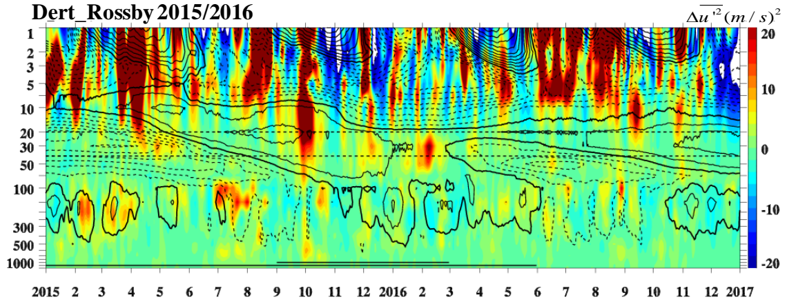
Figure 2. Temporal evolution of Rossby wave activity as squared zonal wind anomalies averaged over 10^\circ\text{S} - 10^\circ\text{N} in the vertical direction. Color shading denotes the anomalies with respect to the monthly climatology (the unit is m^2/s^2 ). The zonal mean zonal wind is overlaid in black contours with contour interval of 5 m/s . The solid and dotted black contours denote westerly and easterly winds, respectively. The thick contours represent the zero wind line. The horizontal dashed lines denote the altitudes of 20 and 40 hPa. The horizontal solid lines denote the El Niño (single line) and strong El Niño periods (double line) in the bottom.
