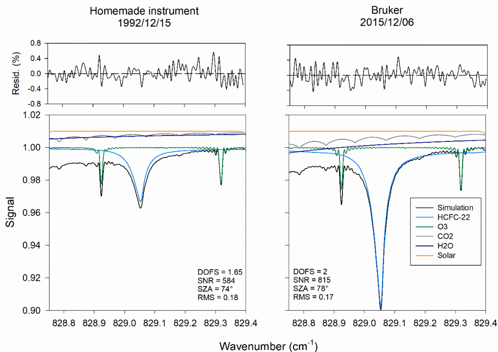
5 Figure 1: Simulations of the 828.5–829.4 cm -1 spectral window from spectra recorded by the homemade (1992/12/15) and Bruker(2015/12/06) FTIR instruments at Jungfraujoch. CO 2 , H 2 O and solar spectra are offset vertically for clarity. Upper frames display relative residuals (%) from the fits to the spectra. These fits are typical of the spectra database in terms of SNR, root mean square error, DOFS and solar zenith angle, regarding their respective year. Note that the lower frame vertical scales correspond to only 10% of the signal amplitude.
