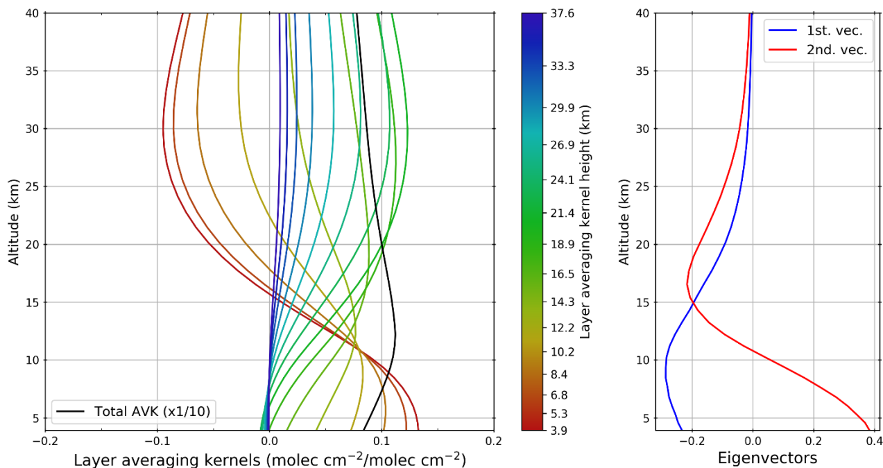
10 Figure 2: Mean layer averaging kernels (left) normalized for partial columns (molec cm -2 /molec cm -2 ) and eigenvectors (right) characterizing the FTIR retrievals of HCFC-22 above Jungfraujoch from spectra recorded in 2015 by the Bruker instrument. The ticks on the colour bar are the individual layer averaging kernels represented in the plot. The first eigenvector has a value of 1 for both instruments, and their second eigenvector has a value of 0.68 and 0.85 for the homemade and Bruker instruments, respectively.
