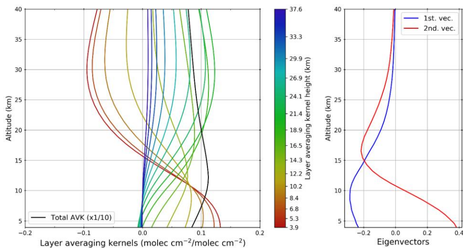
Figure 2: Mean layer averaging kernels (left) normalized for partial columns ( \text{molec cm}^{-2}/\text{molec cm}^{-2} ) and eigenvectors (right) characterizing the FTIR retrievals of HCFC-22 above Jungfraujoch from spectra recorded in 2015 by the Bruker instrument. The ticks on the colour bar are the individual layer averaging kernels represented in the plot. The first eigenvector has a value of 1 for both instruments, and their second eigenvector has a value of 0.68 and 0.85 for the homemade and Bruker instruments, respectively.
