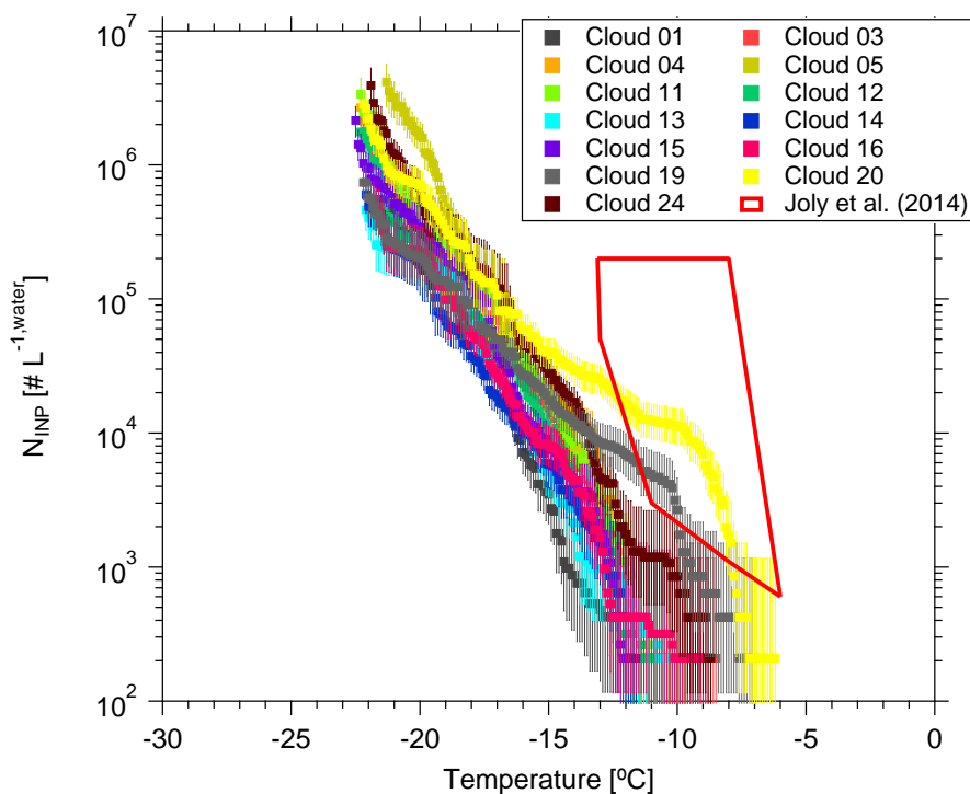
Figure 7. N_{\text{INP}} as a function of temperature in cloud water. Error bars show the 95% confidence interval. Previous field measurements of N_{\text{INP}} in cloud water by Joly et al. (2014) are compared, as shown by the red box.
