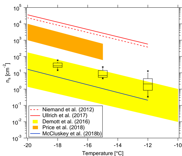
Figure 10. n_s as a function of temperature in this study is shown by black boxes. The boxes represent the interquartile range. Whiskers represent 10th to 90th percentile. Data not included between the whiskers are plotted as an outlier with a star. Two n_s parameterizations (Niemand et al., 2012; Ullrich et al., 2017) for pure desert dust are shown in dashed and solid red lines, respectively. n_s parameterizations from McCluskey et al. (2018b) for pristine SSA over the Northeast Atlantic are shown as a solid blue line. We also compare to recent data from airborne measurement in a dust layer by Price et al. (2018) in brown shadow and from nascent laboratory generated and ambient SSA by DeMott et al. (2016) in yellow shadow, respectively.
