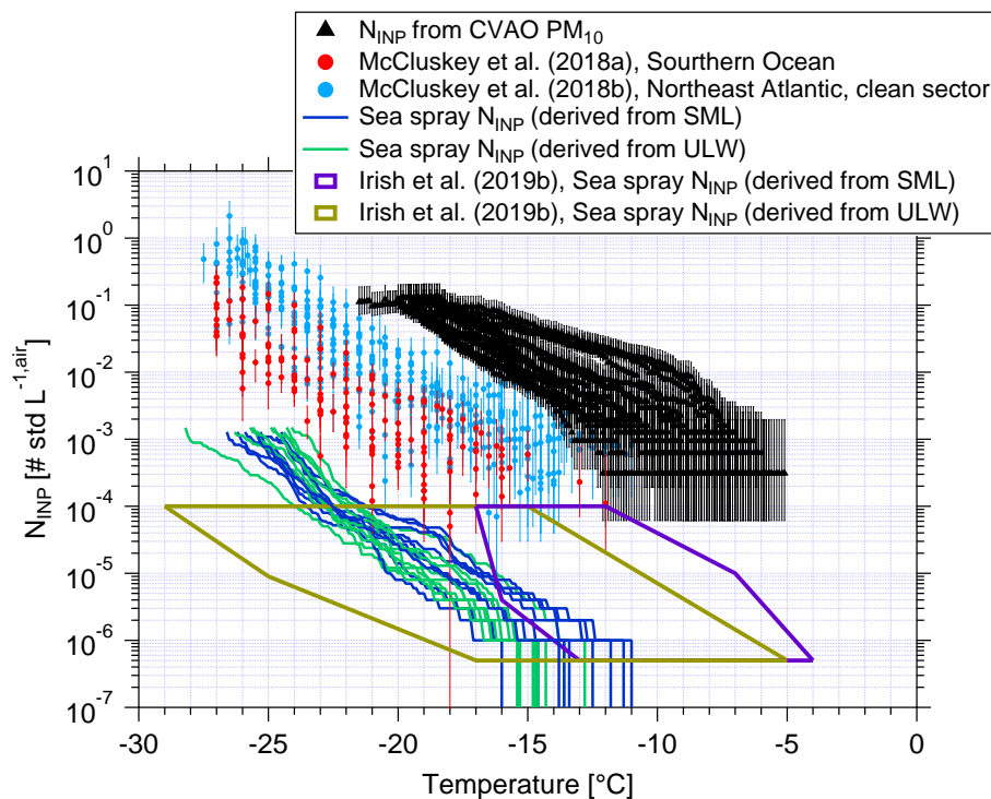
Figure 9. N_{\text{INP}} as a function of temperature from \text{PM}_{10} filters (black triangles), and error bars show the 95% confidence interval. N_{\text{INP}} as a function of temperature from McCluskey et al. (2018a, b) are shown by red and light blue dots, respectively. Error bars show the 95% confidence interval. N_{\text{INP}}^{\text{sea spray,air}} from this study are shown by blue (derived from SML) and green lines (derived from ULW). N_{\text{INP}}^{\text{sea spray,air}} from Irish et al. (2019b) are shown by purple (derived from SML) and brown (derived from ULW) boxes.
