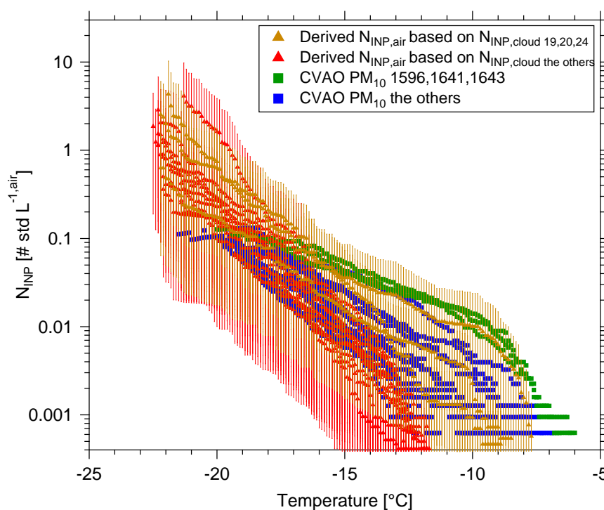
Figure 8. The measured N_{\text{INP}} as a function of temperature in the air by squares. The derived N_{\text{INP,air}} based on INP concentrations measured for cloud water are shown by triangles. The samples with highly ice active INPs at warm temperatures, are shown in a different color than the others: CVAO 1596, CVAO 1641 and CVAO 1643 are shown by green squares and derived N_{\text{INP,air}} based on Cloud 19, Cloud 20 and Cloud 24 are shown by brown triangles. The uncertainty range indicated for the derived N_{\text{INP,air}} originate from calculations with 7 and 20 \mu\text{m} cloud droplet size.
