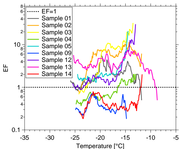
Figure 2. EF as function of temperature. The EF=1 is shown by dashed line.
