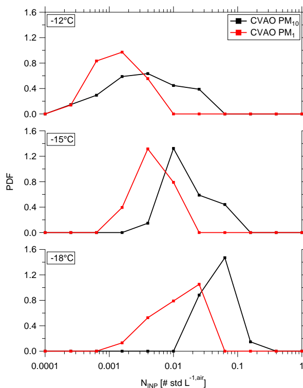
Figure 4. PDFs of N_{\text{INP}} measured from CVAO \text{PM}_{10} filters by black line and CVAO \text{PM}_1 by red line at -12^\circ\text{C} in the upper panel, -15^\circ\text{C} in the middle panel and -18^\circ\text{C} in the lower panel.
