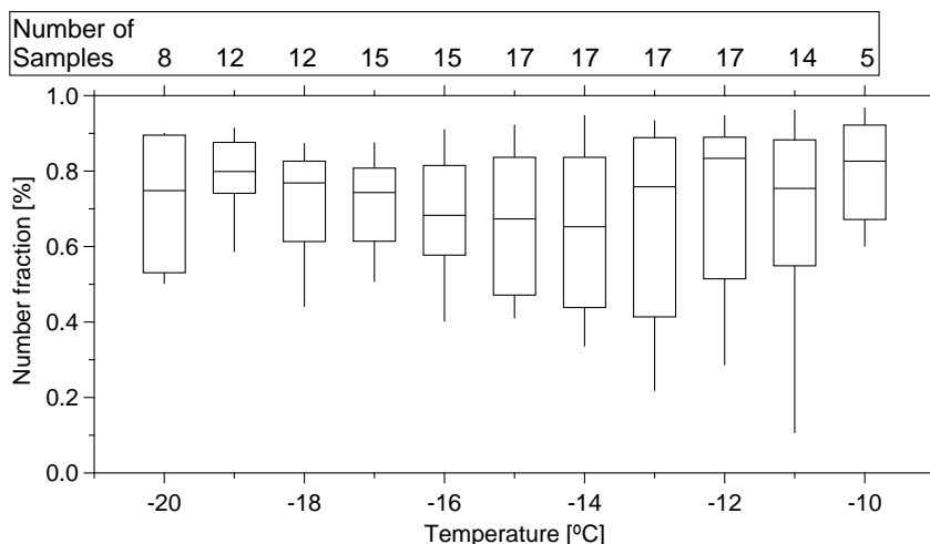
Figure 5. Boxplot of number fraction of INPs in the size range of >1 \mu\text{m} as a function of temperature. The number of samples indicated on top of the figure shows how many different samples contributed at the different temperatures.
