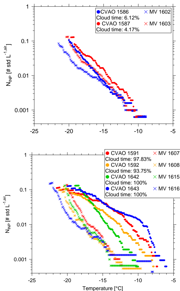
Figure 6. N_{\text{INP}} as a function of temperature from CVAO PM 10 filters and MV PM 10 filters during less (cloud time fraction <10%) cloud effected periods (a) and highly (cloud time fraction >90%) cloud effected periods (b).
