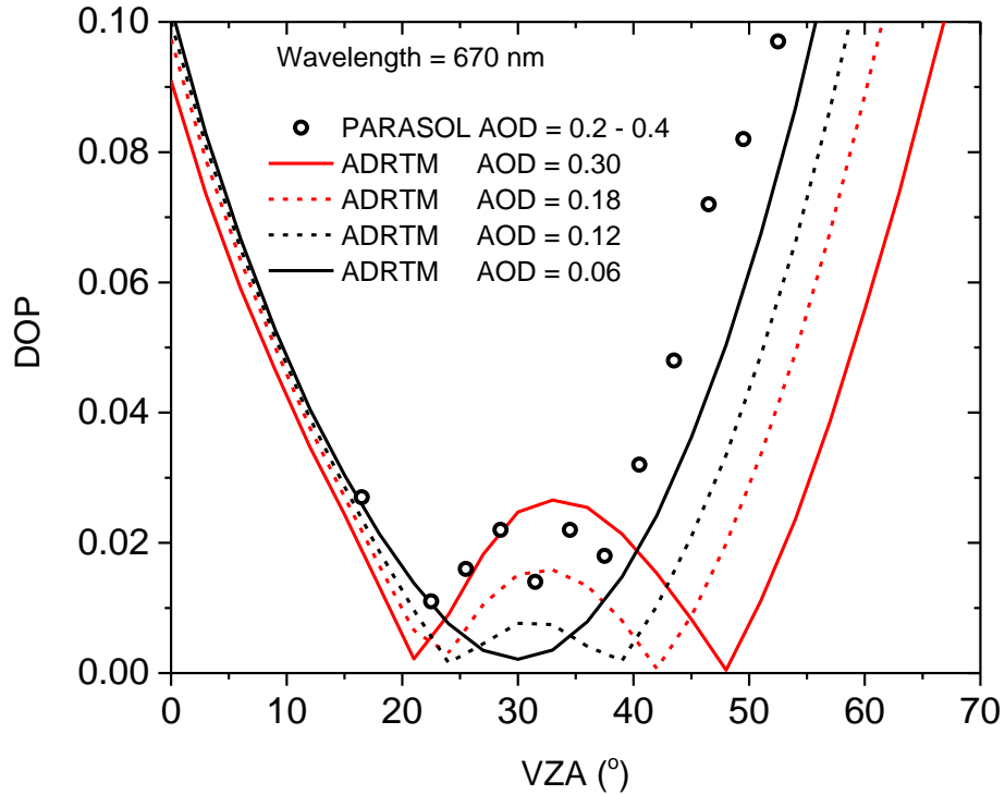
99 100 Figure 1. At near-backscatter angles [For this case, it is at viewing zenith angle (VZA) = ~20-40°, 101 and relative azimuth angle (RAZ) = ~170-180°], the DOP of light from dust monotonically 102 increases with the AOD of dust aerosols. In this modeling, the adding-doubling radiative transfer 103 model (ADRTM) developed in Sun and Lukashin (2013) is used. The wavelength is 670 nm, the 104 solar zenith angle (SZA) is 30°, and wind speed over ocean surface is 7.5 m/s. Also shown in this 105 figure are the PARASOL measurements obtained over Atlantic Ocean area (0°N -35°N and 0°W - 106 60°W) that has Sahara dust. 12 days of PARASOL data in May-August, 2006 are used for this 107 study. The results are for a RAZ of 177°. 108 109
