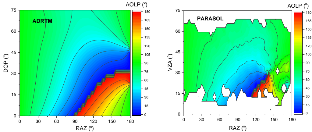
Figure 2. Same as in Fig. 1, but for the AOLP of the reflected light from the ADRTM (left panel, AOD = 0.3) and the PARASOL (right panel, AOD = 0.2 – 0.4).
