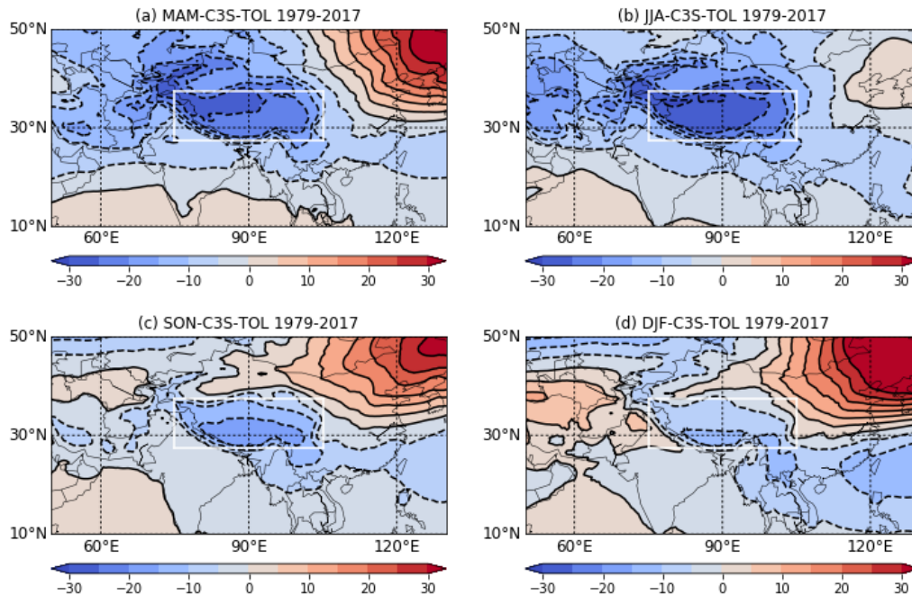
305 Figure 2. Latitude-longitude cross section of the zonal ozone deviations for (a) March-April-May (MAM), (b) June-July-August (JJA), (c) September-October-November (SON) and (d) December-January-February (DJF) seasons based on C3S total ozone dataset for 1979-2017 time period. The solid and dashed contours represent the positive and negative zonal deviations. The contour interval is 5 DU. The TP region ( 27.5^{\circ} - 37.5^{\circ} N, 75.5^{\circ} - 105.5^{\circ} E) is marked by the white rectangle.
