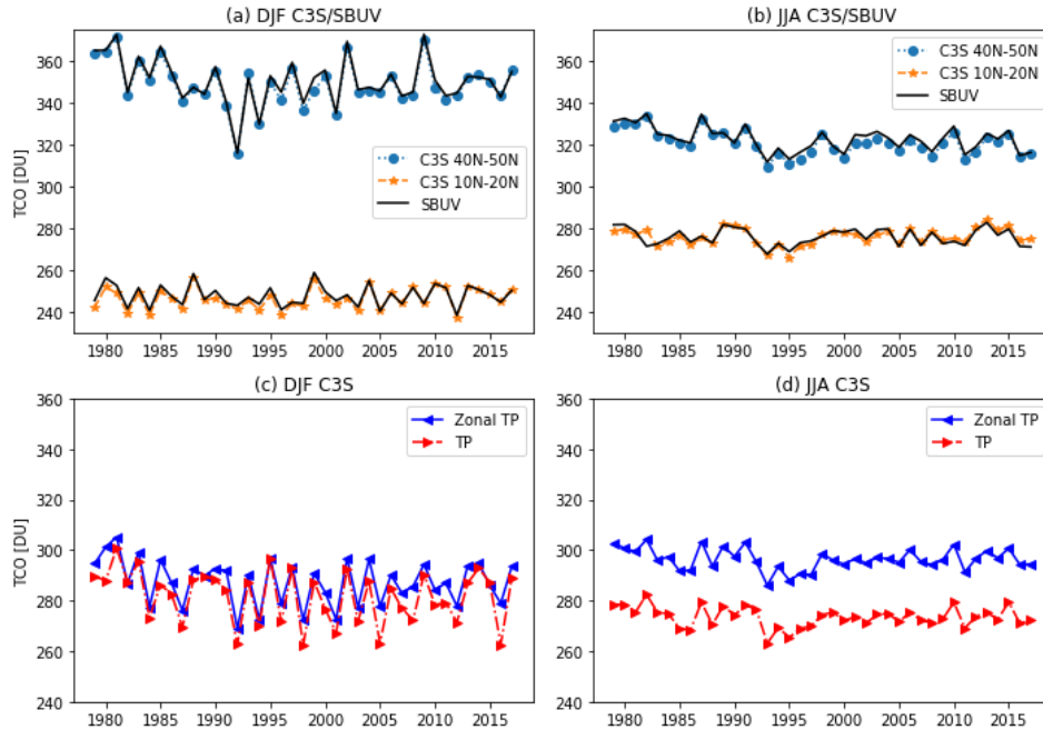
275 Figure 1. C3S-based total column ozone (TCO) time series averaged for December-January-February (DJF) and June-July-August (JJA) seasons during 1979-2017 over (a, b) the North-TP (40 °-50 °N), and South-TP (10 °-20 °N) regions, and (c, d) the zonal-TP (27.5 °-37.5 °N) and the TP regions (27.5 °-37.5 °N, 75.5 °-105.5 °E). Panels (a) and (b) also show the satellite-based observations from SBUV (black solid lines).
