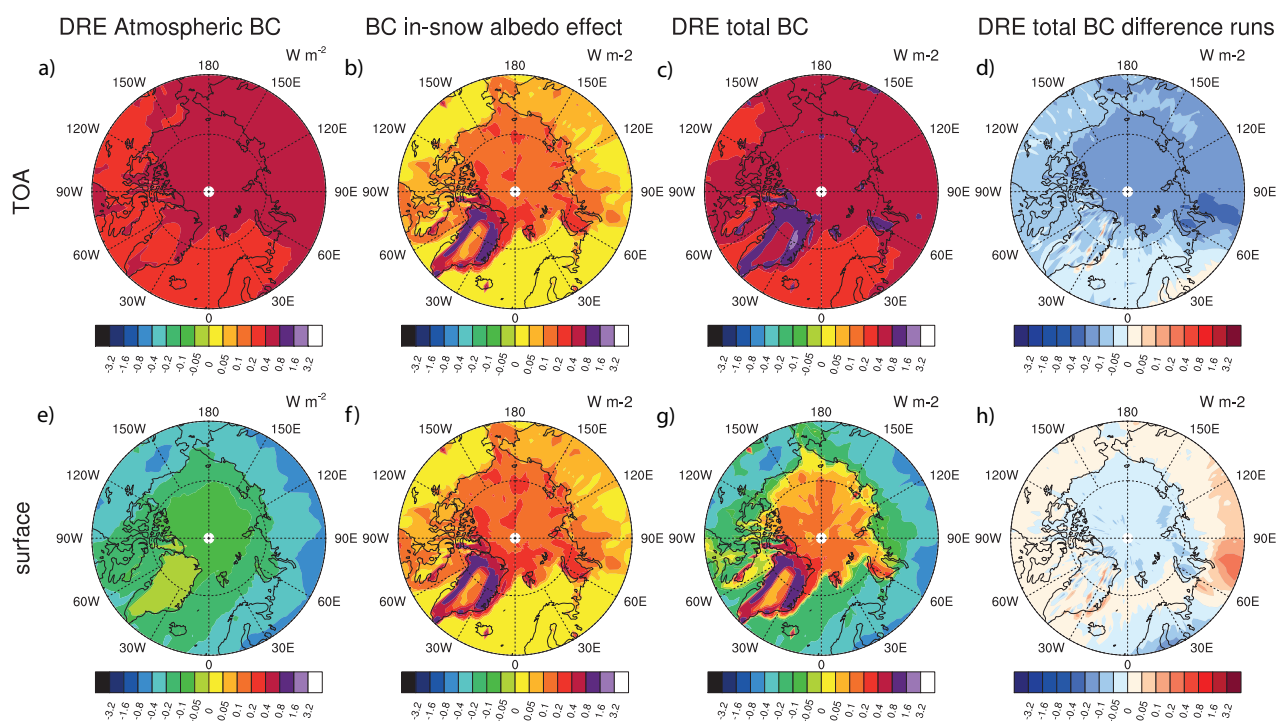
Figure 14. Multi-year mean all sky direct radiative effect (DRE) of BC for the period 2005-2009. Top row for TOA and bottom row for BOA. Panels (a) and (e) show the BCRUS net (terrestrial + solar) DRE of atmospheric BC. Panels (b) and (f) solar BC-in-snow albedo radiative effect. Panels (c) and (g) show the total of the radiative effects of atmospheric and BC deposited in snow (terrestrial plus solar). Panels (d) and (e) show the difference in the total BC radiative effect of the runs ACCMIP-GFAS minus BCRUS.
