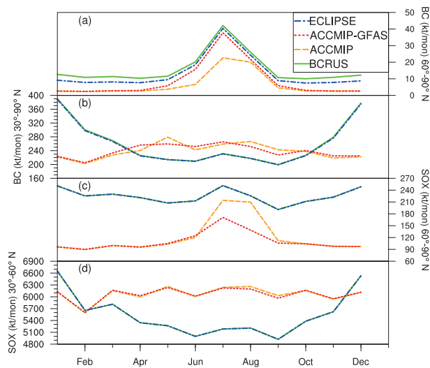
Figure 2. Multi-year monthly mean emissions of (a,b) BC and (c,d) SO x for the years 2005-2015. Values are integrated over the latitude band between 60° N and 90° N, and between 30° N and 60° N, respectively.
