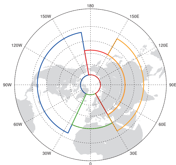
Figure 1. Regions indicate the area used for averaging presented in Table 2. North America in blue, Europe in green, Russia in red and Central Asia in orange.
