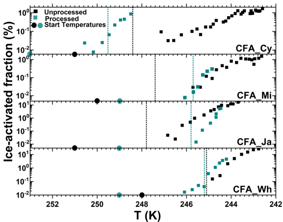
5 Figure 7: Summary of the ice-activated fraction (%) of unprocessed and processed CFA_Cy (5 and 15), CFA_Mi (8 and 23), CFA_Ja (6 and 17), and CFA_Wh (7 and 20) particles as a function of temperature. The number in the brackets are the corresponding experiments numbers in Table 2. The black data points show experiments before the temperature-cycling and freezing (TCF) procedure and the cyan data points represent experiments after the TCF process. The dotted lines correspond to the temperature where water saturation was reached for each experiment.
