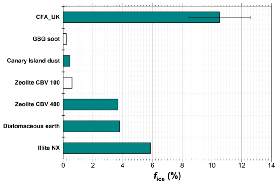
10 Figure 8: Comparison of the ice nucleation enhancement of CFA particles and other particles studied by Wagner et al. (2016). Ice-activated fraction (%) obtained at ~ 250 K start temperature is compared. The filled bars represent ice nucleation via depositional growth while the unfilled bars represent ice nucleation via condensational growth.
