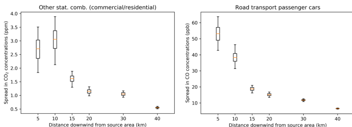
Figure 10: Spread in simulated concentrations of CO 2 resulting from commercial/residential emissions due to uncertainties in the total population proxy map (left) and spread in concentrations of CO resulting from road transport (passenger cars) emissions due to uncertainties in the passenger cars proxy map (right). The box represents the interquartile range, the whiskers the 2.5–97.5 percentile, and the lines the median values of the full ensemble.
