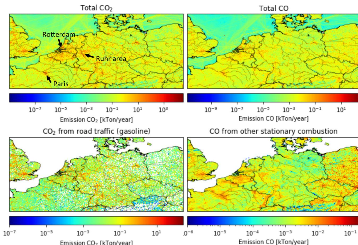
Figure 1: Total emissions of CO 2 and CO, road traffic (gasoline) emissions of CO 2 , and other stationary combustion emissions of CO for 2015 in kt yr -1 (defined per grid cell).
