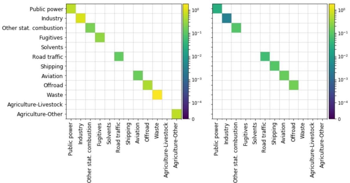
Figure 3: Covariance matrices for spatial proxies (left) and time profiles (right) per aggregated source sector. These are the same for CO 2 and CO. A white space on the diagonal indicates this sector is not included in the Monte Carlo simulation.
