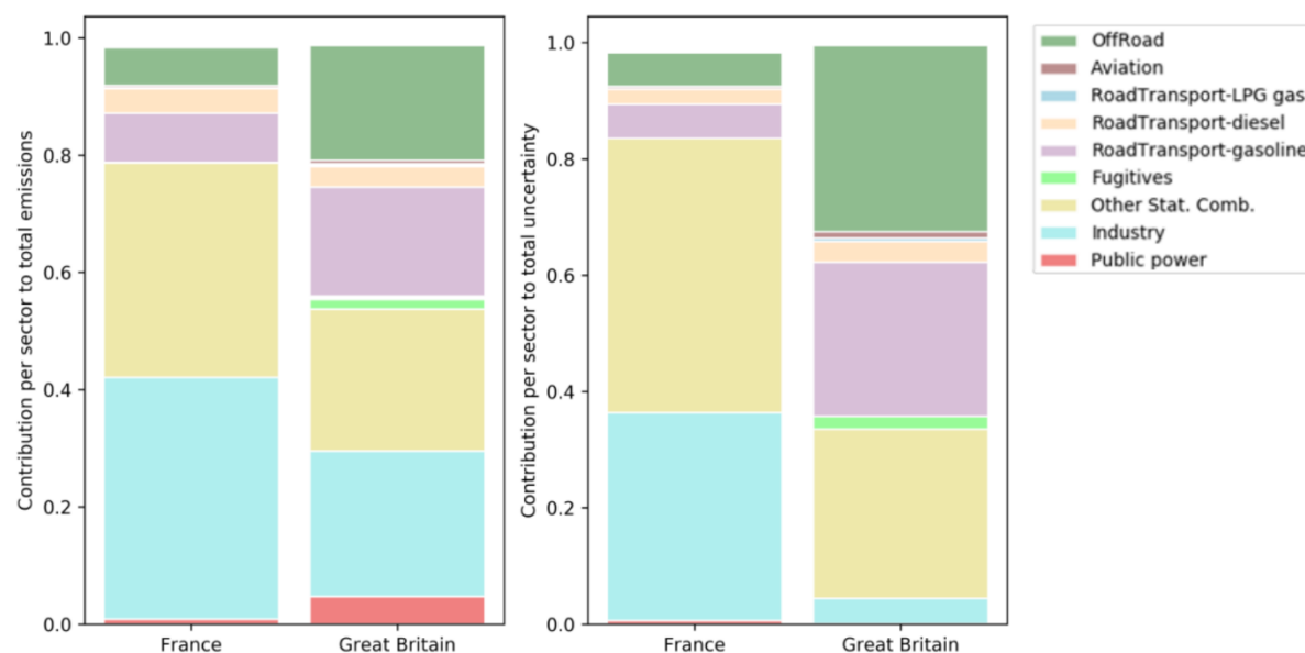
Figure 18: Contribution of source sectors to the total emissions (left) and the total uncertainty (right) in CO for France and Great Britain, summing to 100 %.
