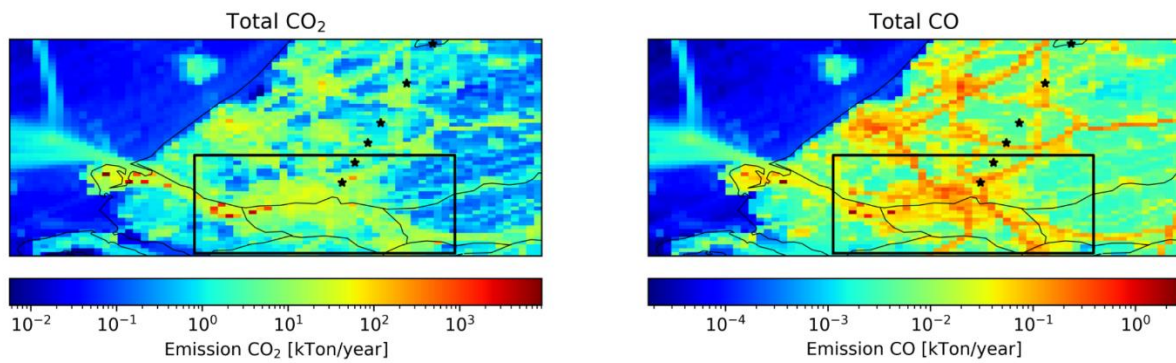
Figure 6: Emissions of CO 2 (left) and CO (right) for part of the Netherlands, including the sub-domain (black rectangle) over Rotterdam. Black stars indicate the receptor locations.
