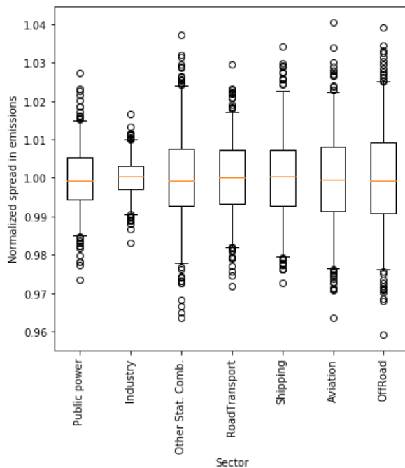
Figure 13: Normalized spread in emissions of CO 2 and CO per sector due to uncertainties in temporal profiles. The box represents the interquartile range, the whiskers the 2.5–97.5 percentile, the lines the median values, and the circles are outliers. The spread is the same for CO 2 and CO, because they have the same temporal profiles.
