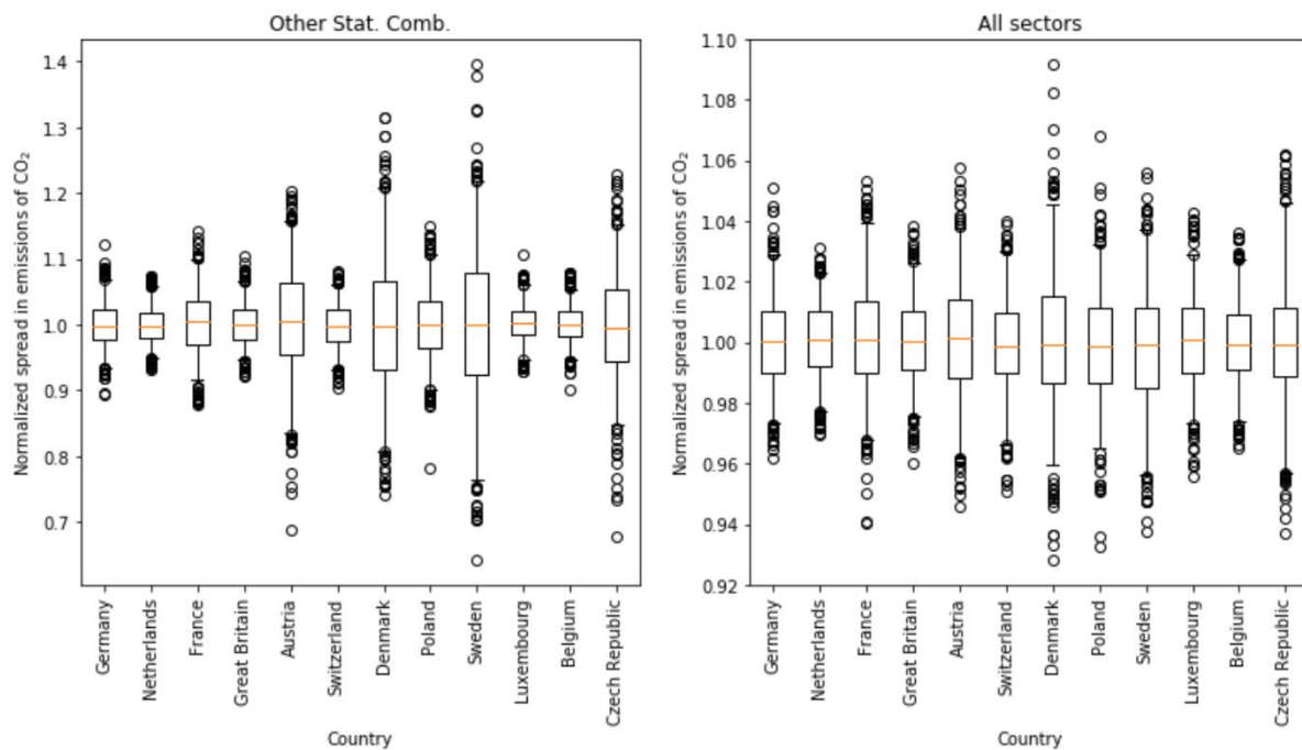
Figure 9: Normalized spread in emissions of CO 2 for other stationary combustion (left) and all sectors combined (right) for a range of countries. The box represents the interquartile range, the whiskers the 2.5–97.5 percentile, the lines the median values, and the circles are outliers.
