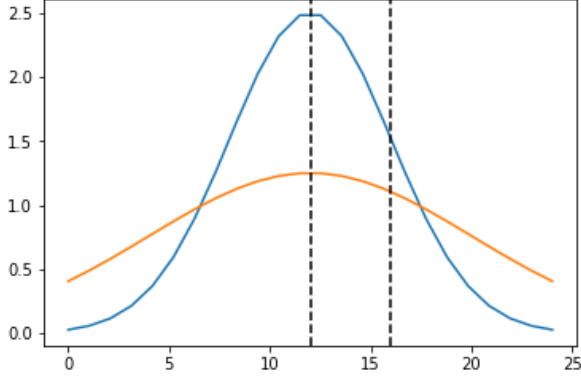
Figure 5: Schematic overview of two possible temporal profiles, which represent a different fraction of the total daily emissions during the selected period (12–16 h LT, illustrated by the dashed lines).
