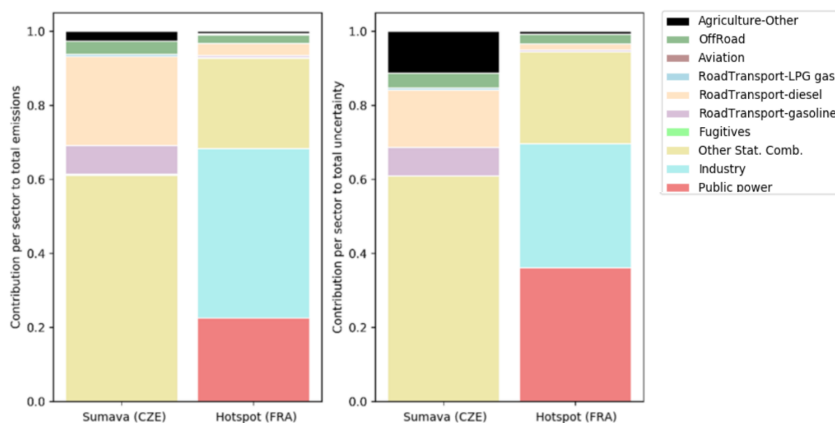
Figure 16: Contribution of source sectors to the total emissions (left) and the total uncertainty (right) in CO 2 for the Sumava national park in the Czech Republic and a hotspot in France, summing to 100 %. See Figure 14 for the exact location of these areas.
