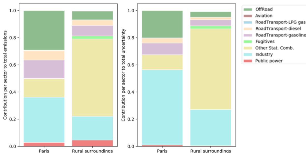
Figure 17: Contribution of source sectors to the total emissions (left) and the total uncertainty (right) in CO for Paris and its surroundings, summing to 100 %. See Figure 15 for the exact location of these areas.
