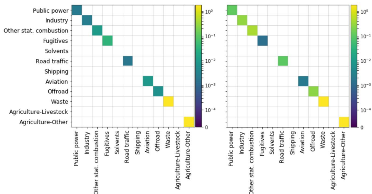
Figure 2: Covariance matrices for total emissions of CO 2 (left) and CO (right) per aggregated source sector. A white space on the diagonal indicates this sector is not included in the Monte Carlo simulation.
