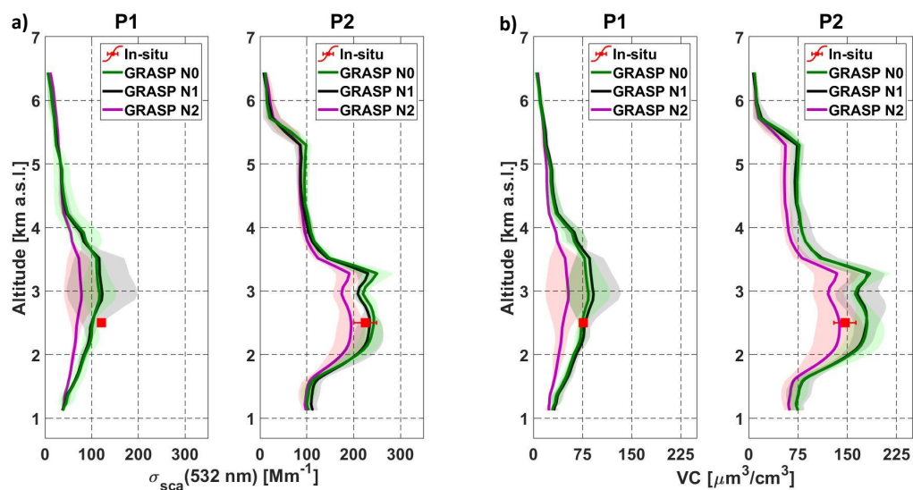
Figure 7. The averaged \sigma_{sca} at 532 nm (a) and VC (b) profiles with its standard deviation (shaded area) retrieved by GRASP N0, N1 and N2 schemes. In red, the averaged in-situ measurements obtained at 2500 m a.s.l. at SNS station.
