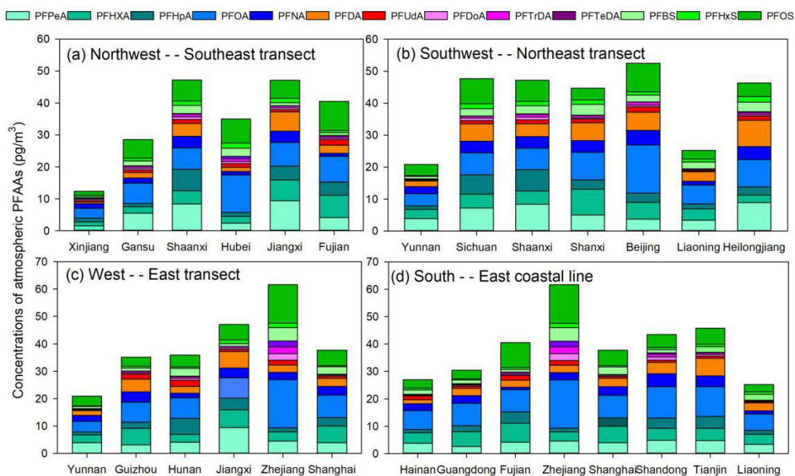
306 307 Fig. 3. Transects of PFAAs concentrations across three different directions and one coastal line
