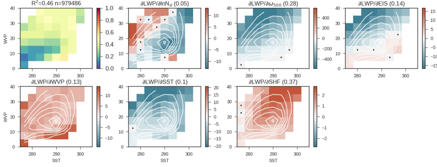
Fig. 6 The regression coefficients relating observed LWP to predictors in the phase space of SST and WVP. Regression coefficients not significant at 99% confidence are marked with a dot. White contours show the distribution of observations in the WVP-SST phase space. The first plot shows the explained variance in each bin. The explained variance within the entire data set is noted in the title along with the number of observations. The remaining plots show the coefficients relating each predictor to LWP. In the title the weighted mean of the absolute value of the standardized coefficient ( \langle \partial \sigma LWP / \partial \sigma x_i \rangle ) is shown in brackets to give an estimate of contribution of each predictor to the variance. Regression coefficients are as described in Eq. 4.
