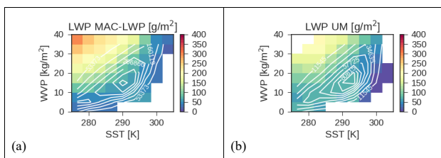
Fig. 2 MAC-LWP observed (a) and UM-simulated (b) LWP in the space of SST and WVP in the region 30°-60°N. White lines show the distribution of data in SST-WVP space. The contours of number of observations in each bin are shown in white.
