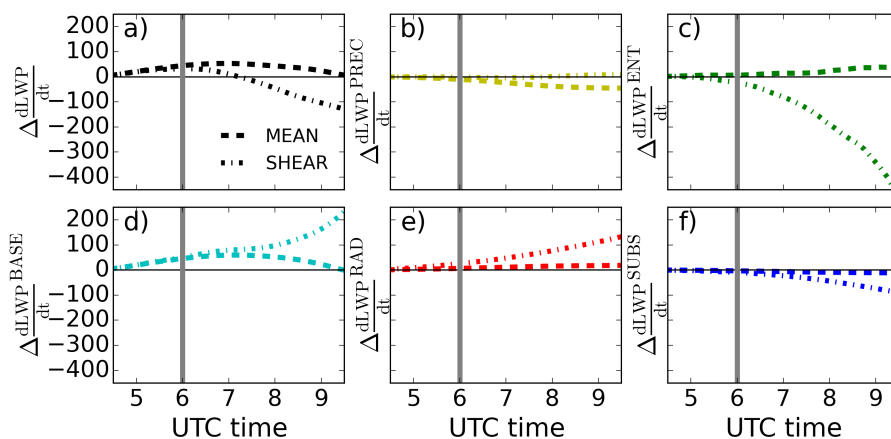
Figure 7. Time series of accumulated differences between MEAN and REF (dashed) and between SHEAR and REF (dotted-dashed) for each term defined in Eq. 2.
