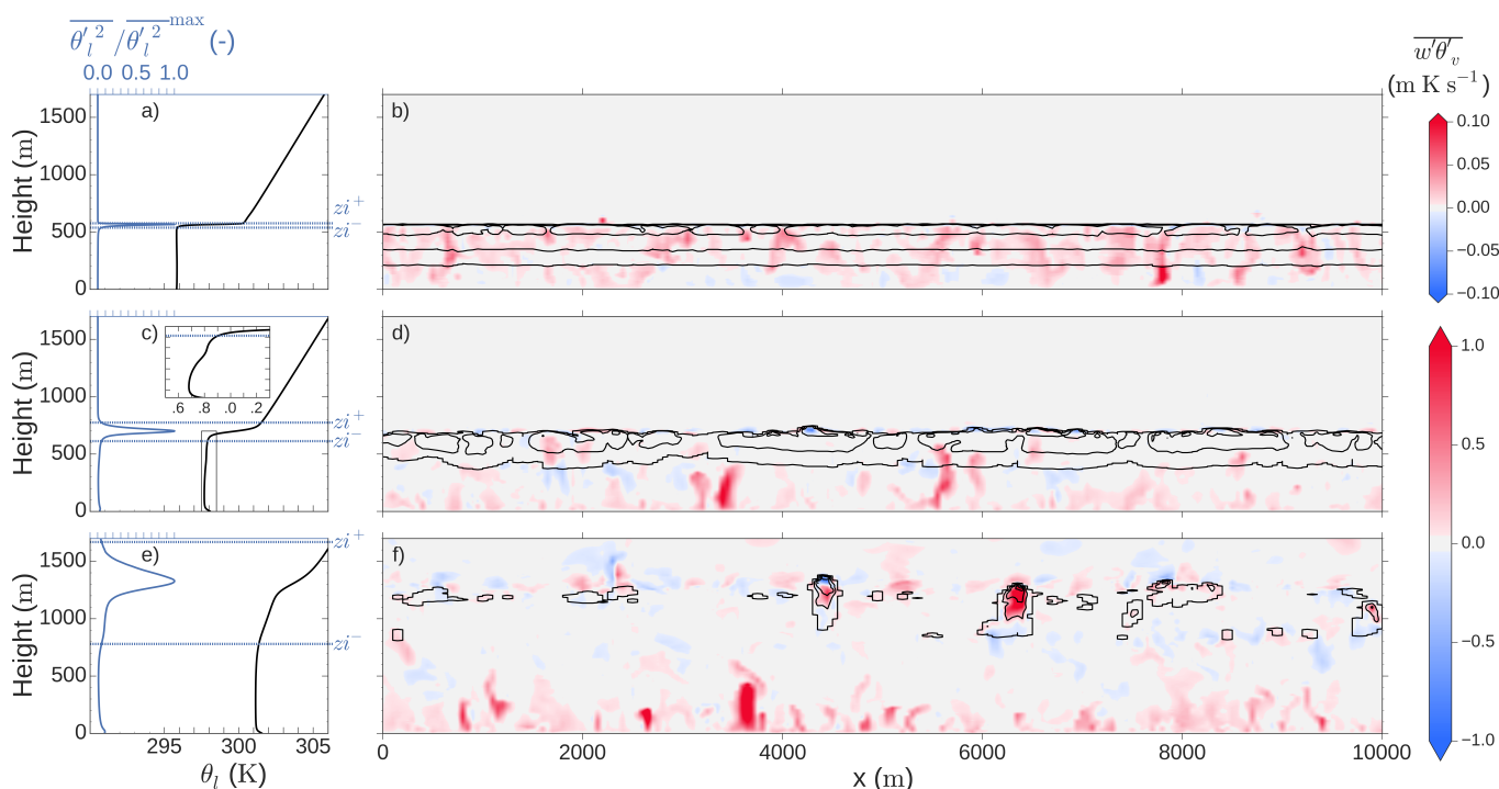
Figure 3. On the left, slab averaged vertical profile of liquid potential temperature \theta_l (black) and \overline{\theta_l'^2} normalized over its maximum value (blue). The inversion layer upper z_i^+ and lower z_i^- limits are indicated in dashed blue horizontal lines. On the right, horizontal cross-section of buoyancy flux \overline{w'\theta_v'} (in colours, red (blue) indicating upwards (downwards) movement of buoyantly positive (negative) air) and cloud liquid water (in black contour lines every 0.3 \text{ g}_w \text{ Kg}_a^{-1} ). Top plot corresponds to 05 00 UTC, center to 11 00 UTC and bottom to 14 30 UTC. The inset at c) is an expanded version of the rectangle in the same subfigure.
