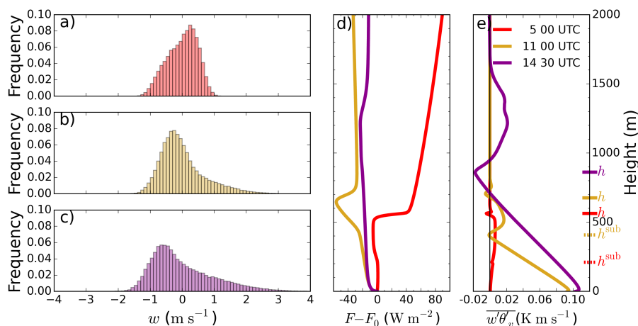
Figure 4. On the left, frequency distribution of vertical velocities at \frac{h}{2} at 5 00 UTC (top), 11 00 UTC (center) and 14 30 UTC (bottom). On the center (d), vertical profile of slab net radiative flux normalized over the surface value at 5 00 UTC (red), 11 00 UTC (dark yellow) and 14 30 UTC (purple). On the right (e) and following the same color code, slab averaged buoyancy flux \overline{w'\theta'_v} . The subcloud layer height h^{\text{sub}} and the boundary layer height h are shown for each time at the right vertical axis in (e). At 14 30 UTC both heights coincide.
