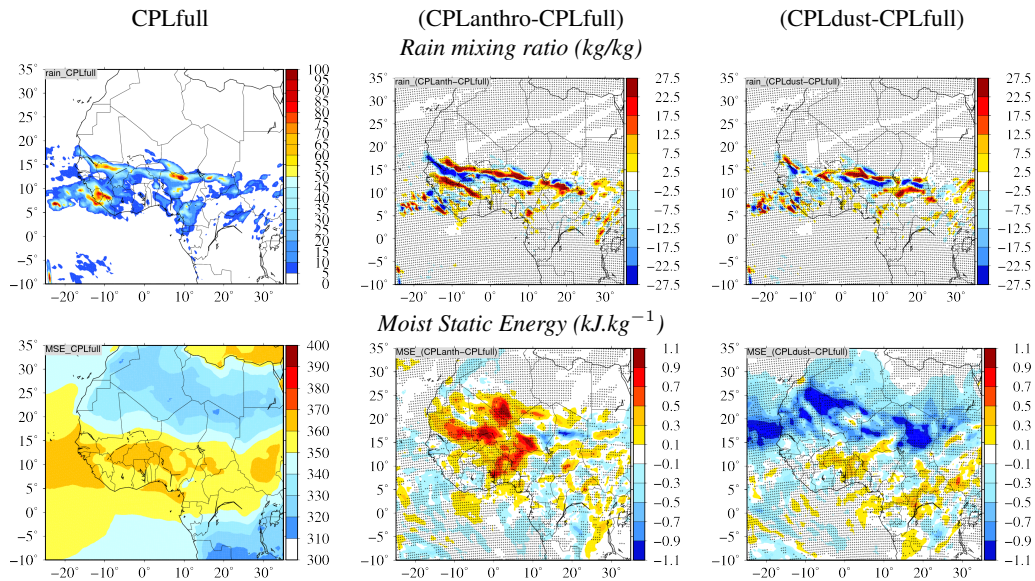
Figure 8. Left column (from top to bottom): Maps of monthly mean rain mixing ratio ( kg/kg ) and moist static energy ( kJ.kg^{-1} ) for July 2016. Middle column: maps of monthly mean of daily averaged differences between CPLanthro and CPLfull for same variables as the left row. Right row: maps of monthly mean of daily averaged differences between CPLdust and CPLfull for same variables as the left row. The tiny crosses on the map indicate where the difference was found to be significant.
