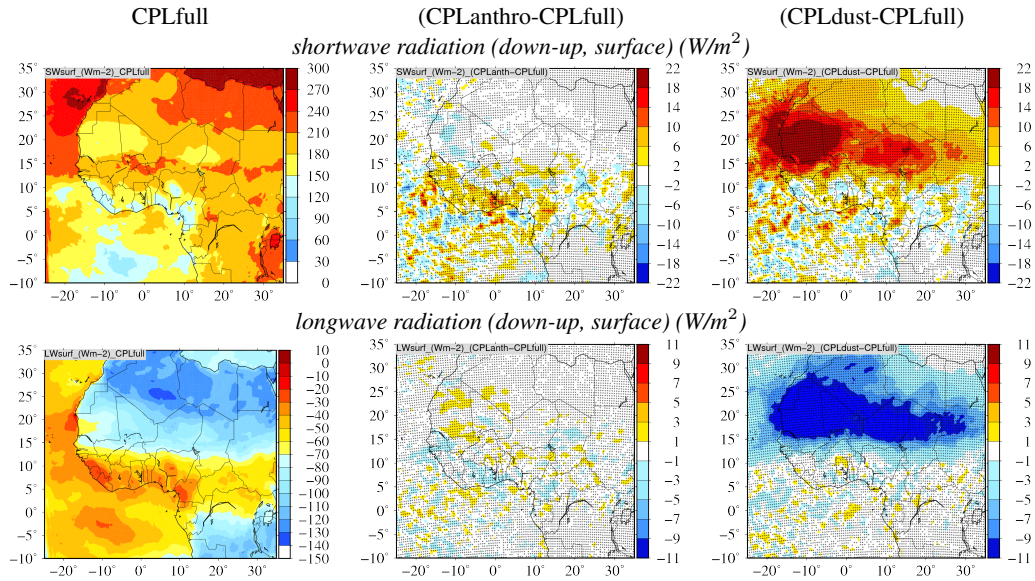
Figure 7. Left column (from top to bottom): Maps of monthly mean shortwave radiation (down-up, surface) ( W/m^2 ) and longwave radiation (down-up, surface) ( W/m^2 ) for July 2016. Middle column: maps of monthly mean of daily averaged differences between CPLanthro and CPLfull for same variables as the left row. Right row: maps of monthly mean of daily averaged differences between CPLdust and CPLfull for same variables as the left row. The tiny crosses on the map indicate where the difference was found to be significant.
