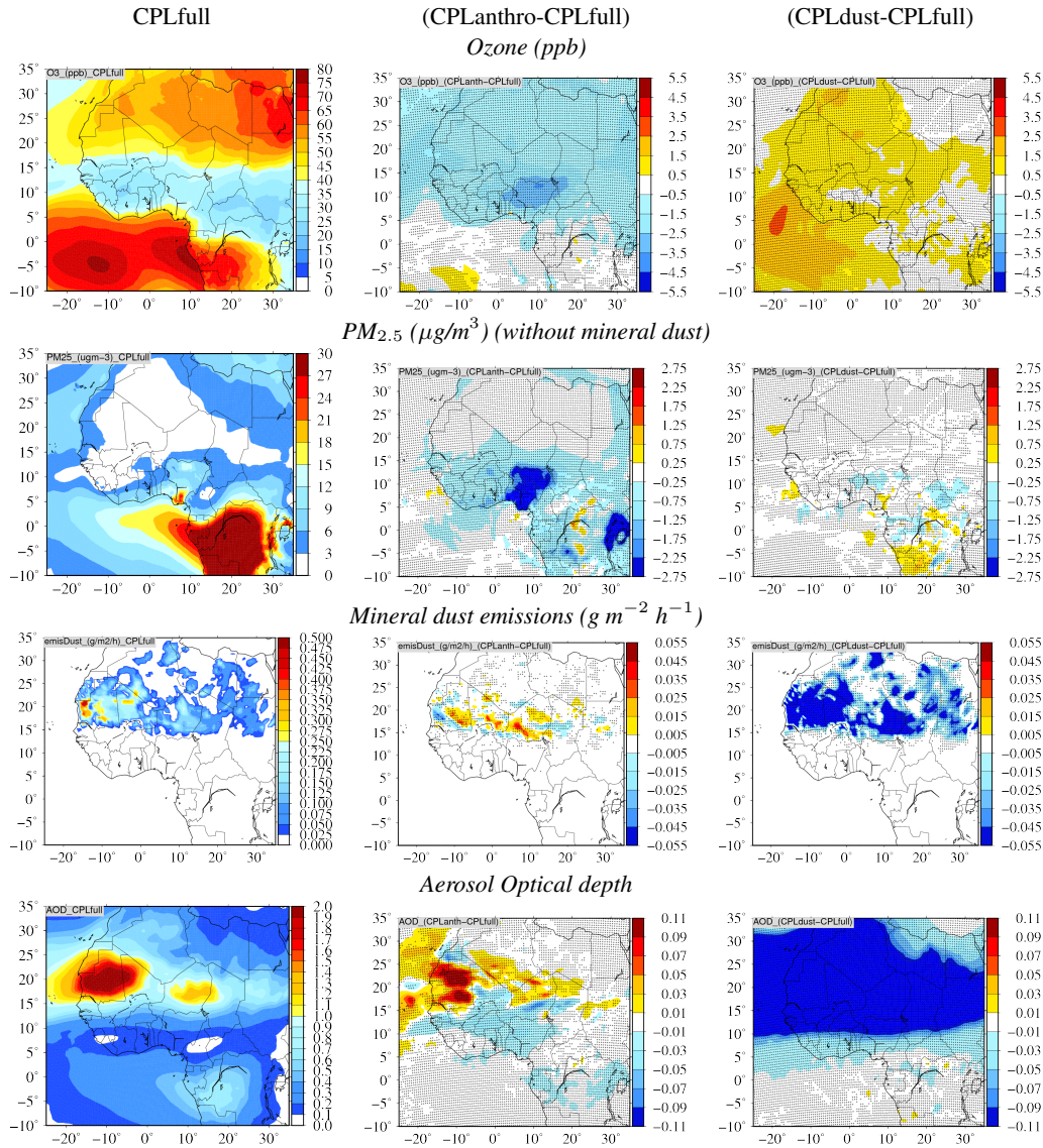
Figure 9. Left column (from top to bottom): Maps of monthly mean of ozone (ppb), PM 2.5 (µg/m 3 ) (without mineral dust), mineral dust emissions (g m -2 h -1 ) and Aerosol Optical depth for July 2016. Middle column: maps of monthly mean of daily averaged differences between CPLanthro and CPLfull for same variables as the left row. Right row: maps of monthly mean of daily averaged differences between CPLdust and CPLfull for same variables as the left row. The tiny crosses on the map indicate where the difference was found to be significant.
