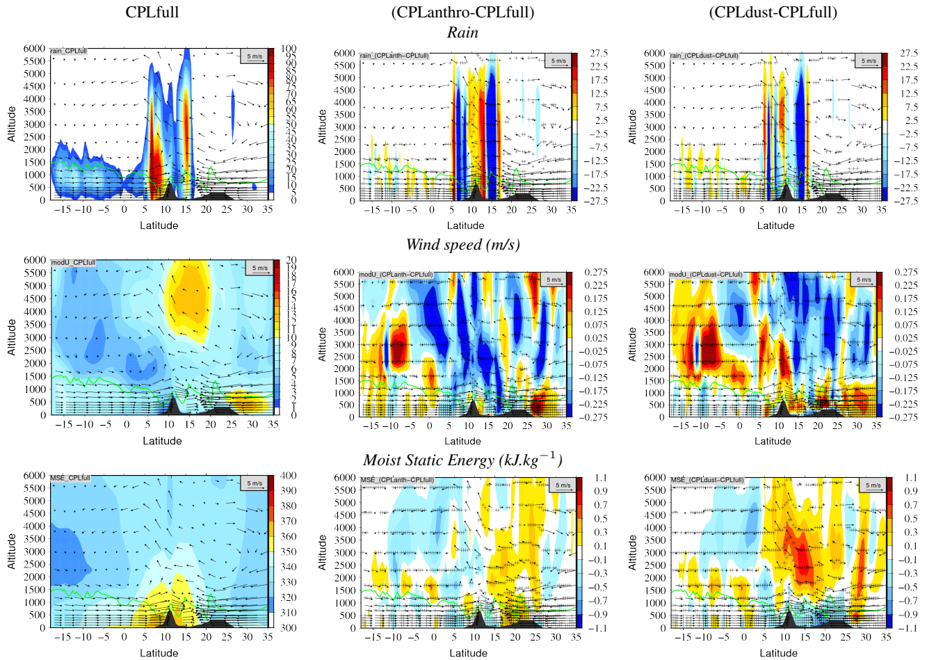
Figure 10. Vertical cross-section of rain and wind speed vertical profiles, averaged from 1 to 31 July 2016 and for longitude -10^\circ . The mean value for CPLfull and the differences (CPLanthro-CPLfull) and (CPLdust-CPLfull) are presented. Crosses indicate locations where the differences are significant.
