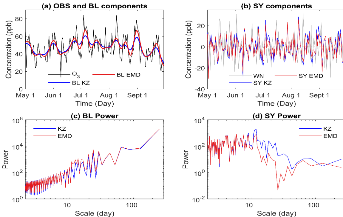
Figure 2. The top left panel displays the raw daily maximum 8-hour ozone time series together with the baselines extracted from the KZ filter and EMD while the top right panel reveals the similarity between white noise and synoptic forcing imbedded in these observed ozone time series. The bottom two panels compare the power spectra of the baseline forcing (left) and the synoptic forcing (right) derived from KZ filtering and EMD (sum of IMF 1 and IMF2). Notice that most of the energy in the baseline time series is in the longer time scale while most of the energy of the short-term component is in the high-frequency range. The similarity of results from both scale separation techniques demonstrates that the two scales of interest (i.e., baseline and synoptic forcing) have been extracted reasonably well.
