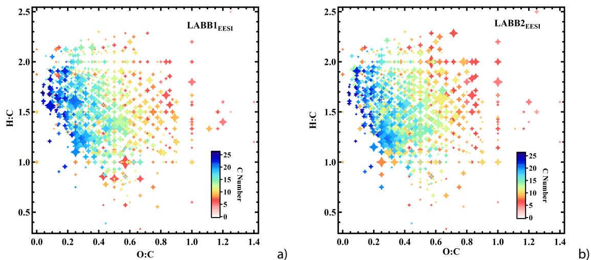
Fig. 4. a), b) Van Krevelen plot (atomic H:C vs. O:C ratio) of the LABB1 EESI and LABB2 EESI factor mass spectra. Points are sized by the fraction of each neutral compound apporportioned to LABB1 EESI and LABB2 EESI and colored by number of carbon atoms.
