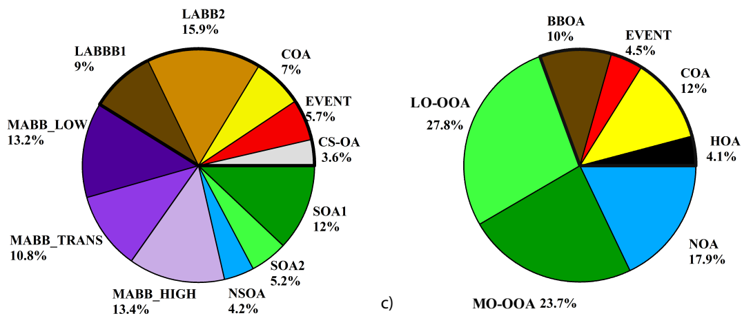
Fig. 14. Comparison between EESI factors and AMS factors: time series of the mass flux of each EESI PMF factors (a) and time series of concentrations of each AMS PMF factors (b). Pie charts of source apportionment results from the EESI (left) and AMS (right) (c). The thick block frame denotes the sum of the primary OA for both data sets.
