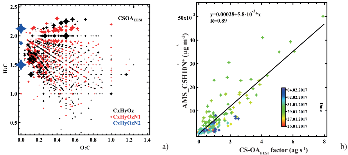
5 Fig. 5. a) Van Krevelen plot (atomic H:C vs. O:C ratio) of the cigarette smoking (CS-OA EESI ) factor mass spectrum. Points are sized by the fraction of each neutral compound apportioned to CS-OA EESI . Colors denote C x H y O z , C x H y N 1 O z , and C x H y N 2 O z groups. b) Comparison of CS-OA EESI and C 5 H 10 N + AMS , colored by time.
