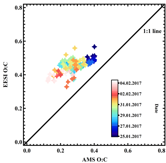
Fig. 13. Comparison of EESI-TOF and AMS. Total EESI-TOF mass flux ( \text{ag s}^{-1} ) as a function of AMS OA, points are colored by date (a) and the fraction of levoglucosan (b). The EESI-TOF and AMS comparison in terms of H:C (c) and O:C (d), points are colored by date.
