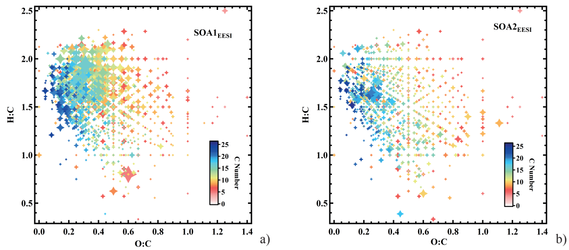
Fig. 9 Van Krevelen plots (atomic H:C vs. O:C) for the SOA1 EESI and SOA2 EESI factor mass spectra. The points are sized by the fraction of each neutral compounds apportioned to SOA1 EESI and SOA2 EESI and colored by the number of carbon atoms.
