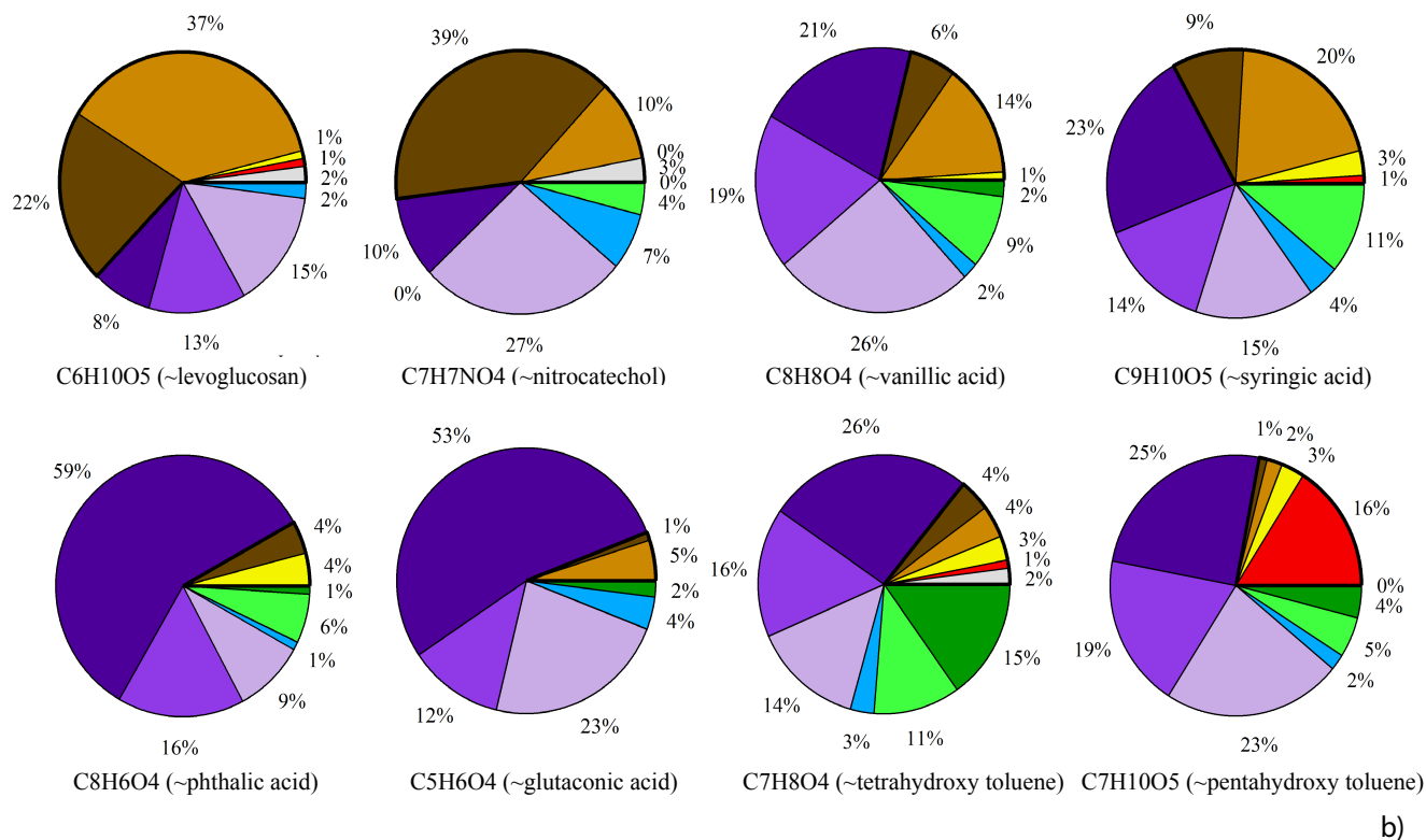
Fig. 10. Apportionment of selected ions by EESI-TOF PMF. (a) Time series of the mass flux ( \text{ag s}^{-1} ) and (b) mean fraction apportioned to each factor. Each ion is associated with a compound of interest having this molecular formula, however, the relative isomeric abundance of this compound cannot be confirmed by the EESI-TOF.
