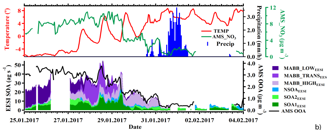
Fig. 6. Factor profiles (a) and stacked time series (b) of the 6 EESI-TOF SOA PMF factors, together with AMS OOA. The latter panel also shows meteorological data. All EESI-TOF data are plotted in mass flux ( \text{ag s}^{-1} ), AMS in \mu\text{g m}^{-3} , other units are included. Factor profiles (b) are molecular weighted and are normalized such that the sum of each profile is 1.
