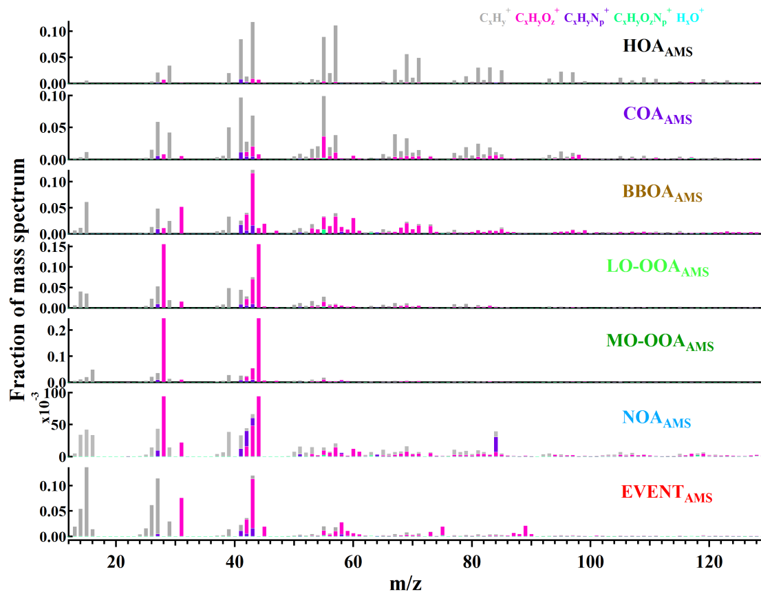
5 Fig. 1. Factor profiles for the 7-factor AMS PMF solution. \text{HOA}_{\text{AMS}} is constrained by a -value 0.1. The total signal of each factor is normalized to unity. ( \text{HOA}_{\text{AMS}} : Hydrocarbon OA, \text{COA}_{\text{AMS}} : Cooking-related OA, \text{BBOA}_{\text{AMS}} : Biomass burning OA, \text{OOA}_{\text{AMS}} : Oxygenated OA, \text{NOA}_{\text{AMS}} : Nitrogen containing OA, \text{EVENT}_{\text{AMS}} , an isolated local event)
