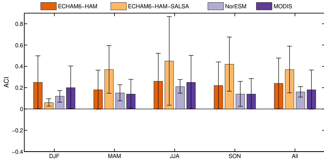
Figure 7. Global (over land only) estimates of the aerosol-cloud interaction (ACI) computed as the changes of \ln(\text{CDNC}) to \ln(\text{AI}) . CDNC are derived from corresponding daily grid points of LWP and COT from MODIS observations and COSP-MODIS outputs following Bennartz (2007). ACI values are calculated by season and for the entire period (1 January 2008 – 31 December 2008). Uncertainties estimates are calculated as 95% confidence interval from the daily values.
