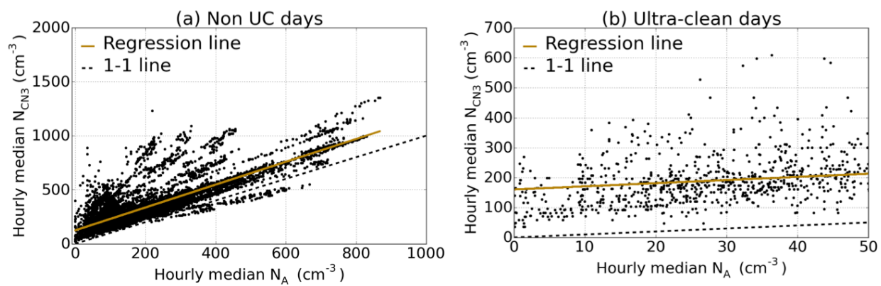
Figure S1: Hourly median N_{CN3} is regressed against hourly median N_A for both (a) non ultra-clean days and (b) ultra-clean days.
