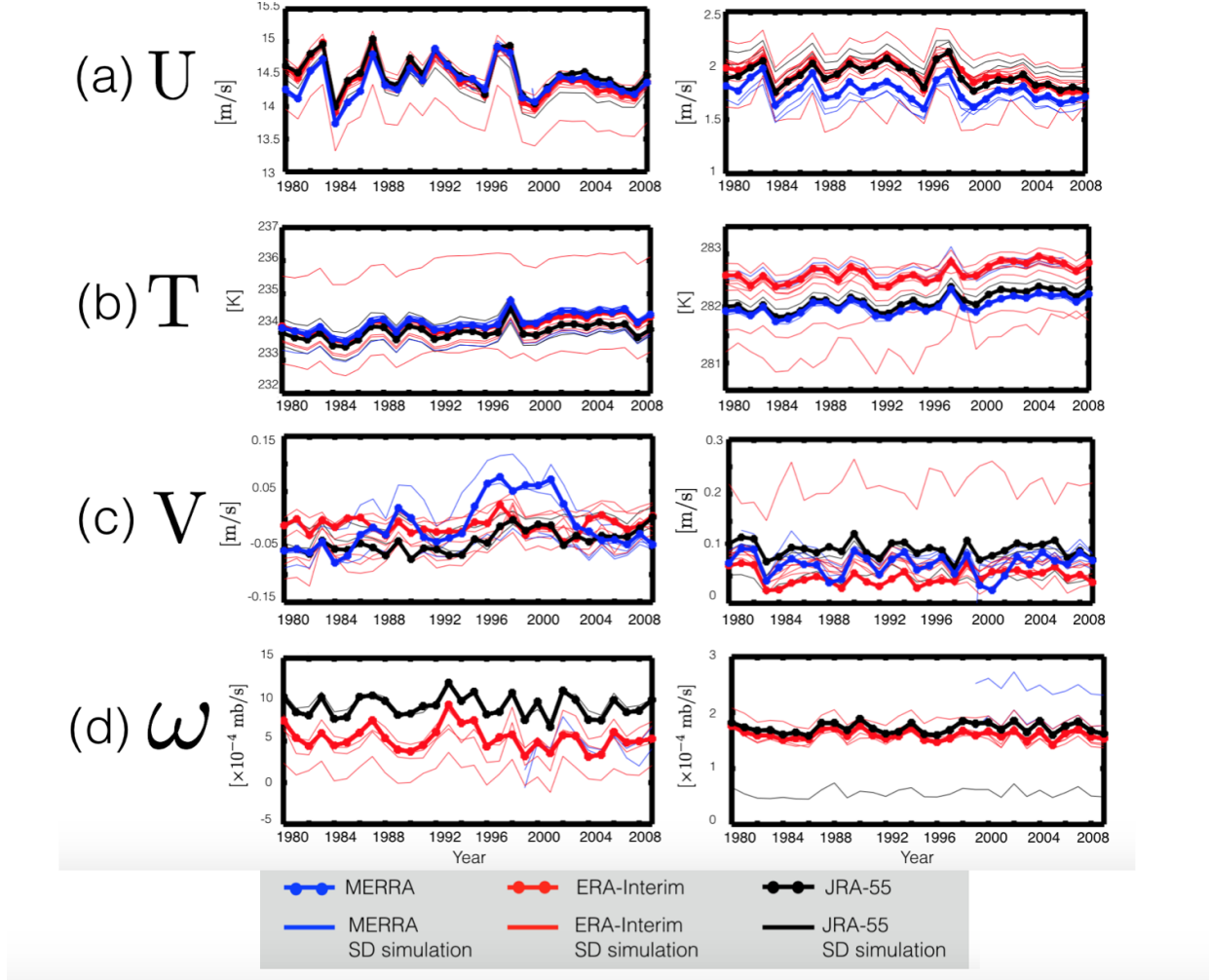
Figure 7. Timeseries of the zonal mean zonal winds (a), zonal mean temperatures (b), zonal mean meridional winds (c) and zonal mean vertical velocities (d) at 300 hPa (left panels) and 850 hPa (right panels). Red/blue/black solid lines correspond to SD simulations constrained with ERA-Interim/MERRA/JRA-55 reanalysis fields. Red/blue/black dotted lines correspond to the raw ERA-Interim/MERRA/JRA-55 meteorological fields. MERRA assimilated fields are shown for all variables, except for \omega , for which output was not available.
