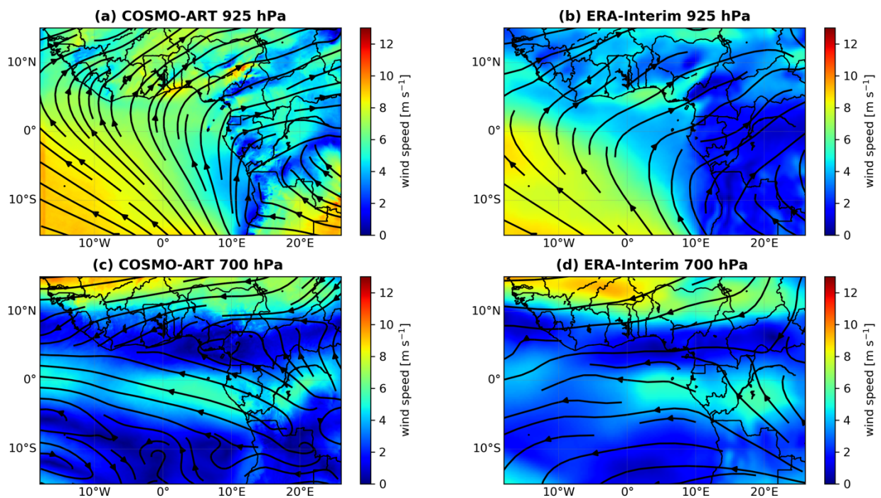
235 Figure 2. Average wind speed (color shading) and streamlines at 925hPa (top) and 700hPa (bottom) simulated with COSMO-ART (left) and in ERA-Interim re-analysis (right) for July 2016. Note the different scales in top and bottom panels.
