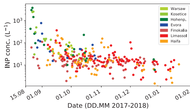
Figure 6. Ice-nucleating particle (INP) concentration estimated from the smoke extinction coefficients in Fig. 4(c), assuming heterogeneous ice nucleation (deposition nucleation) on soot particles at the temperature T = -55^\circ\text{C} and a typical ice supersaturation level during cirrus formation of S_{\text{ice}}=1.15 (Ullrich et al., 2017).
