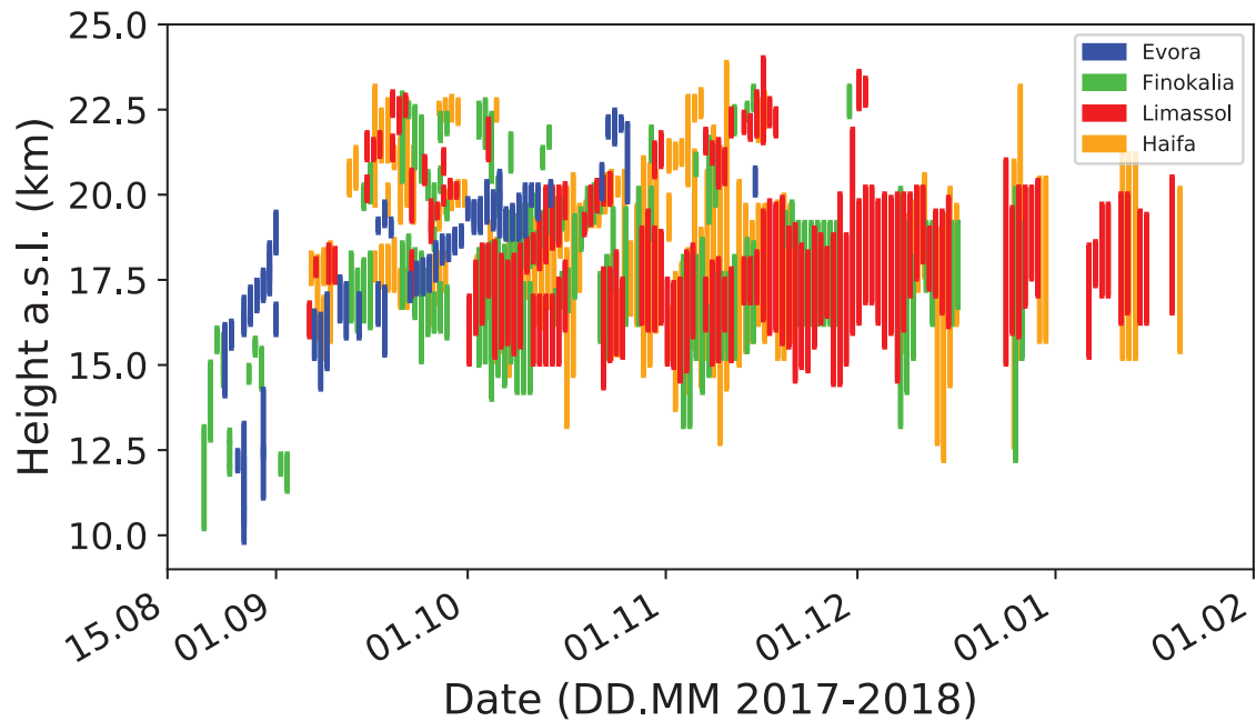
Figure 8. Same as Fig. 4a, except for the southern Polly stations only. The Finokalia data set is shown here in green for better identification. The different data sets are shifted against each other by 6 hours and the linewidth is reduced to better see all observations. An ascending structure, first seen over Evora in September (in blue) and then also detected over the Eastern Mediterranean in October and November (in green, red, and orange) triggered the discussion about potential aerosol lifting processes and effects.
