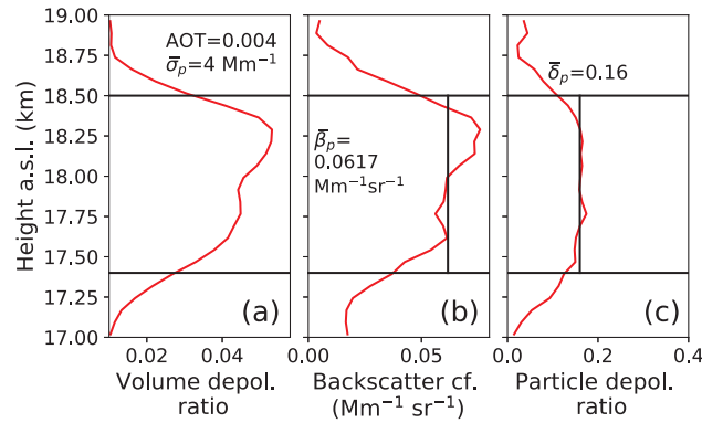
Figure 2. Analysis of a Polly measurement at Limassol, Cyprus, on 9 September 2017. The 532 nm backscatter and depolarization ratio profiles are computed from six-hour mean lidar return signal profiles (18:00-24:00 UTC). Vertical signal smoothing with a window length of 367.5 m is applied. The volume depolarization ratio in (a) and the particle backscatter coefficient in (b) were used to identify the smoke layer. The shown smoke layer base and top heights (horizontal lines) are mean values for the observation period, estimated from subsequent 60-90-minute mean depolarization ratio profiles. The particle depolarization ratio in (c) is the one for smoke (after the correction for Rayleigh depolarization contributions). Values for the vertically averaged particle extinction coefficient \overline{\sigma_p} (for the column from z_{\text{bot}} and z_{\text{top}} , assuming a lidar ratio of 65 sr) and 532 nm AOT, mean backscatter coefficient \overline{\beta_p} , and mean particle linear depolarization ratio \overline{\delta_p} are stated in the three panels, respectively.
