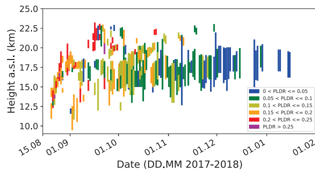
Figure 7. All individual day-by-day smoke observations of the 532 nm particle linear depolarization ratio (from all contributing stations, including several Lindenberg observations at 355 nm). Colors indicate different depolarization value ranges. The depolarization ratio decreased with time because of the removal of the larger non-spherical smoke particles and/or the change in the shape characteristics (from non-spherical to spherical particle shape).
