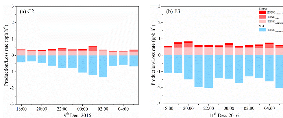
Figure 11. Separated contributions of production and loss terms (colored bars) of HONO on (a) the 9 th (C2) and (b) 11 th (E3) of December 2016. An upper limit uptake coefficient for NO 2 was adopted to calculate the HONO production rate on aerosol surface.
