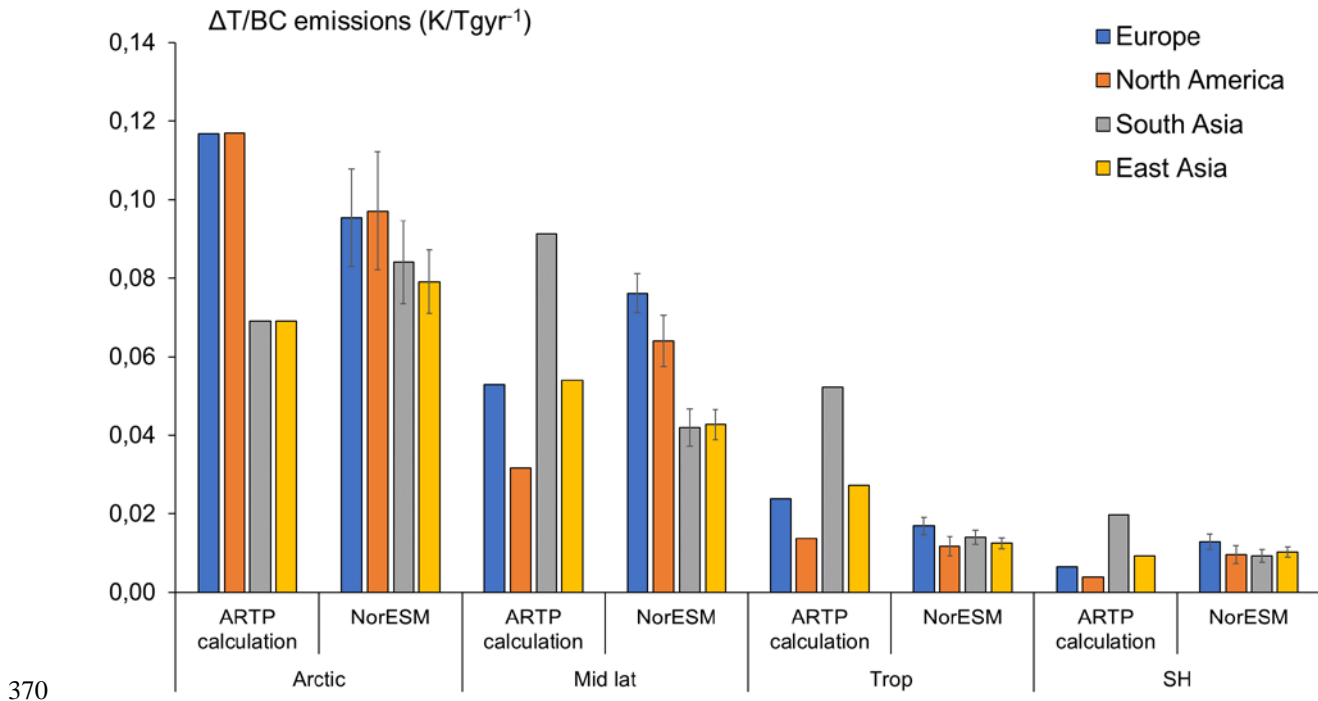
Figure 7: A comparison between ARTP calculated and NorESM calculated regional surface temperature response per unit BC emissions (K/Tgyr -1 ). The lowest emission perturbation is shown here (10×Europe, 10×North America, 10×South Asia, 5×East Asia). The response region (latitude band) is given on the x-axis. The error bars for NorESM represent the standard error of mean.
