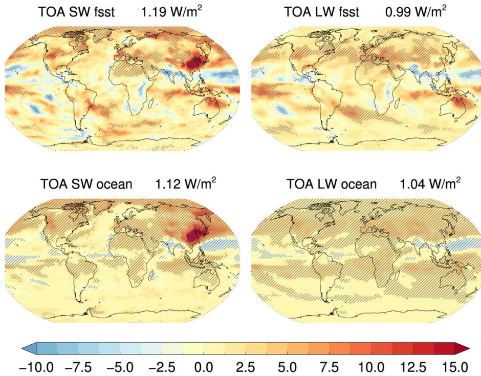
360 Figure 5: Change in delta TOA net SW and LW radiative fluxes (sum of downward and upward) for the 10xBC in East Asia perturbation minus the baseline. Top row shows the runs with fixed SSTs, and bottom row shows the runs with fully coupled ocean. The stippled areas represent statistically significant changes ( p < 0.05 ).
