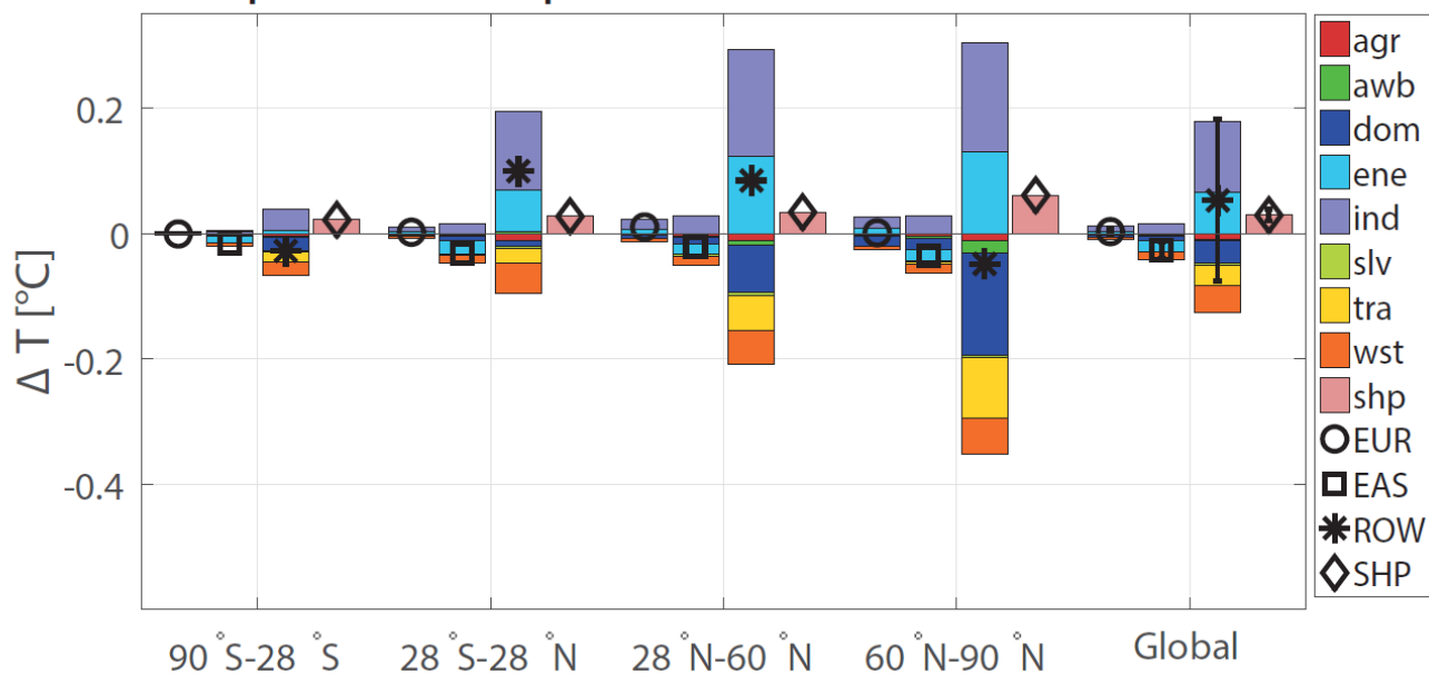
B) Temperature response in 2050, MTFR - CLE
