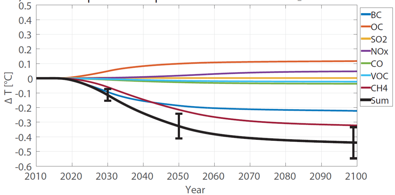
B) Global temperature response difference for MTFR - CLE
