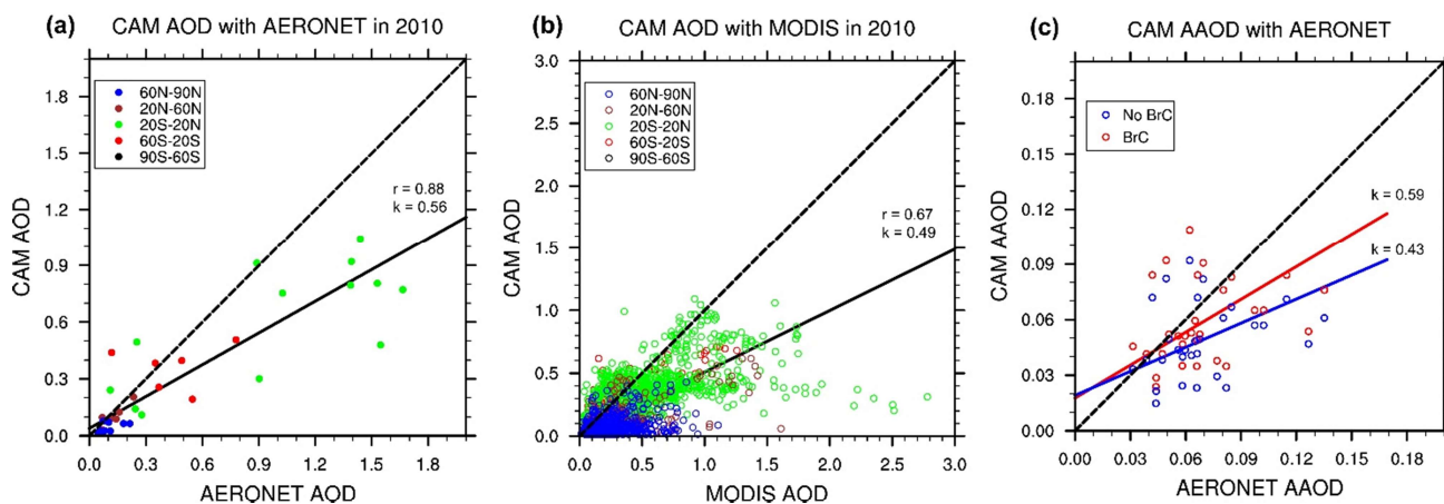
Figure 6. Comparison of monthly mean AOD and AAOD data in 550 nm for fire dominated months and regions (Figure S1(a)) of model simulations with the observations for (a) 2010 AERONET AOD; (b) 2010 MODIS AOD and (c) 2005-2014 AERONET AAOD. For (a) and (b), model data correspond to the same time and location of the observations. The data points in (a) and (b) are color-coded as a function of latitude. The solid line denotes a PC regression line and the dashed line denotes the 1:1 reference line. For (c), monthly mean values of model data corresponding to AERONET AAOD observations are shown. The solid lines denote PC regression lines for model results with and without BrC absorption, and the corresponding regression slope ( k ) values are shown. The dashed line denotes the 1:1 reference line.
