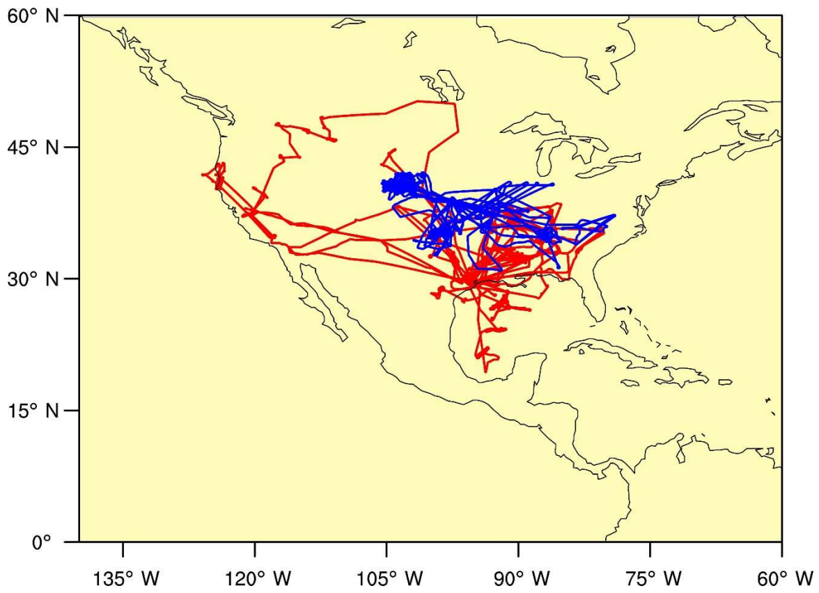
Figure 7. Flight tracks of SEAC 4 RS (red) and DC3 (blue) field experiments.
