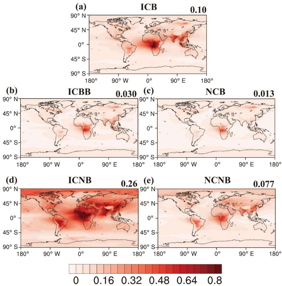
895 Figure 11. Annual averaged global distributions of BrC DRE for all sensitivity simulations (Table 2). The unit is \text{W m}^{-2} . The global averaged DRE is shown in the upper right corner.
