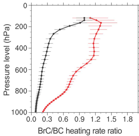
Figure 14. Global averaged vertical profile of BrC to BC heating rate ratio for 2010. The black and red lines are the average profiles for regions without and with deep convection events, respectively. Standard deviations are indicated by the horizontal bars.
