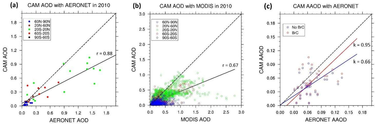
Figure 6. Comparison of monthly mean AOD and AAOD data in 550 nm for fire dominated months and regions (Figure S1(a)) of model simulations with the observations for (a) 2010 AERONET AOD; (b) 2010 MODIS AOD and (c) 2005-2014 AERONET AAOD. For (a) and (b), model data correspond to the same time and location of the observations. The data points in (a) and (b) are color-coded as a function of latitude. The solid line denotes a least-squares regression and the dashed line denotes the 1:1 reference line. For (c), monthly mean values of model data corresponding to AERONET AAOD observations are shown. The solid lines denote PC regression lines for model results with and without BrC absorption, and the corresponding regression slope ( k ) values are shown. The dashed line denotes the 1:1 reference line.
