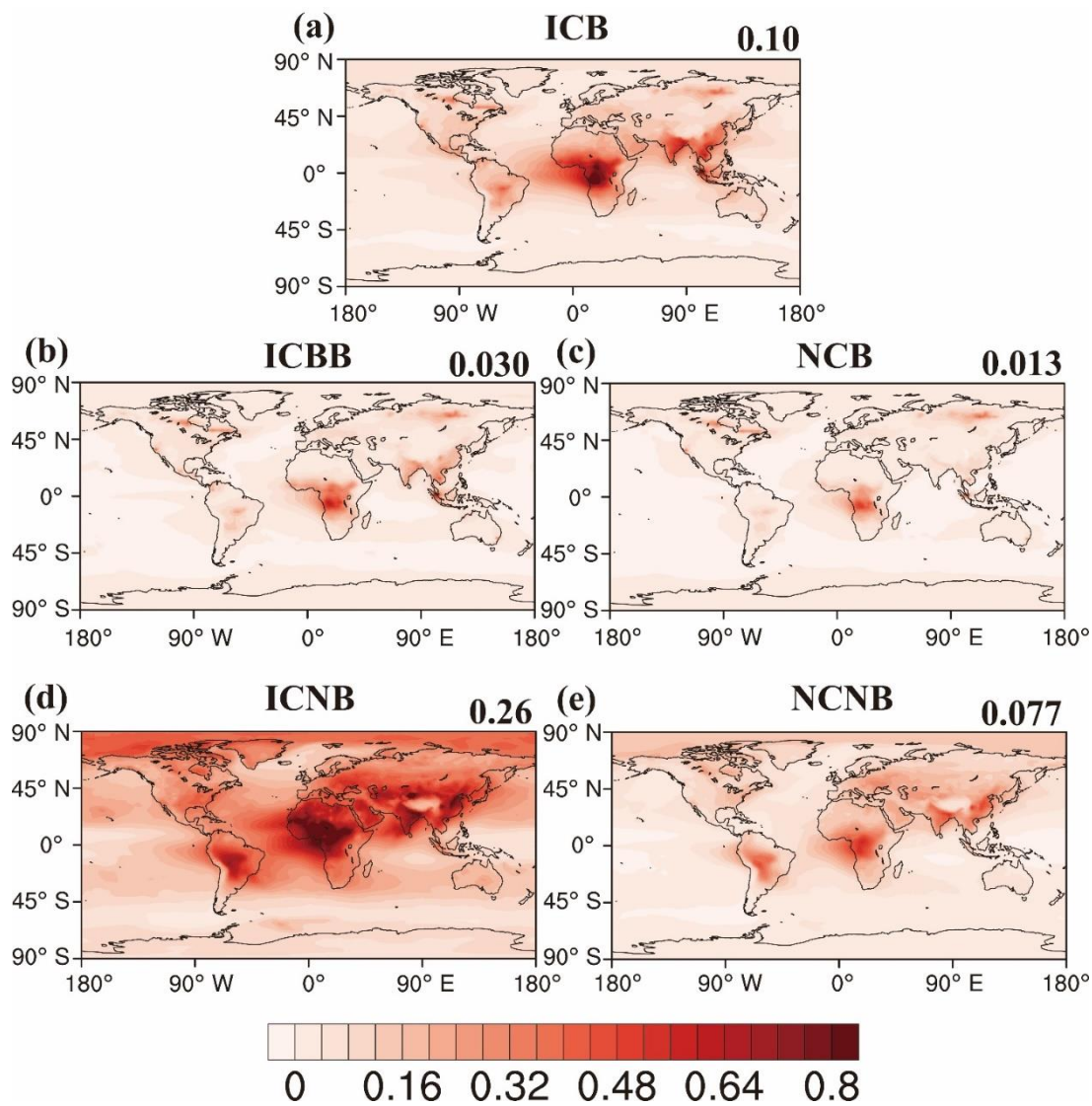
Figure 10. Annual averaged global distributions of BrC DRE for all sensitivity simulations (Table 2). The unit is W m^{-2} . The global averaged DRE is shown in the upper right corner.
