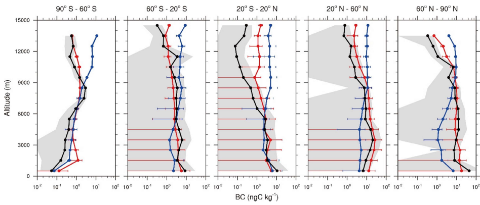
Figure 5. Comparison of observed and simulated BC vertical profiles during HIPPO missions for the latitude bins of 90° S-60° S, 60° S-20° S, 20° S-20° N, 20° N-60° N and 60° N-90° N. Black lines and shaded areas show the means and standard deviations of the observations binned in 1-km intervals, respectively. The colored vertical lines and horizontal bars show the means and standard deviations of the default (blue) and modified CAM5 results (red), respectively.
