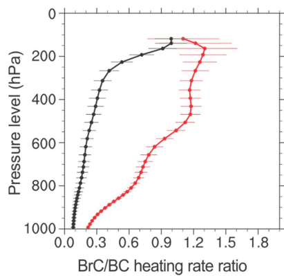
915 Figure 14. Global averaged vertical profile of BrC to BC heating rate ratio for 2010. The black and red lines are the average profiles for regions without and with deep convection events, respectively. Standard deviations are indicated by the horizontal bars.
