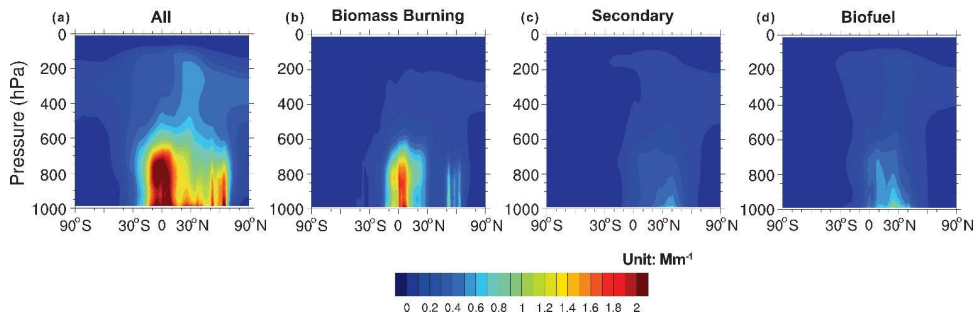
Figure 9. Simulated zonal averaged annual mean BrC absorption at 365 nm ( \text{Mm}^{-1} ) for (a) all sources, (b) biomass burning emissions, (c) secondary BrC formation, and (d) biofuel BrC emissions. Unit is \text{Mm}^{-1} . Color bar is in log scale.
