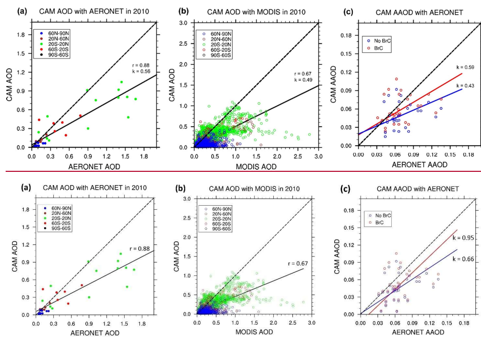
870 Figure 6. Comparison of monthly mean AOD and AAOD data in 550 nm for fire dominated months and regions (Figure S1(a)) of model simulations with the observations for (a) 2010 AERONET AOD; (b) 2010 MODIS AOD and (c) 2005-2014 AERONET AAOD. For (a) and (b), model data correspond to the same time and location of the observations. The data points in (a) and (b) are color-coded as a function of latitude. The solid line denotes a PC least-squares regression line and the dashed line denotes the 1:1 reference line. For (c), monthly mean values of model data corresponding to AERONET AAOD observations are shown. The solid lines denote PC regression lines for model results with and without BrC absorption, and the corresponding regression slope ( k ) values are shown. The dashed line denotes the 1:1 reference line. 875
