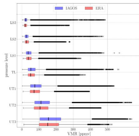
Figure 3. Vertical profile of H 2 O volume mixing ratio [ppmv] for IAGOS (left, blue) and ERA (right, red).
