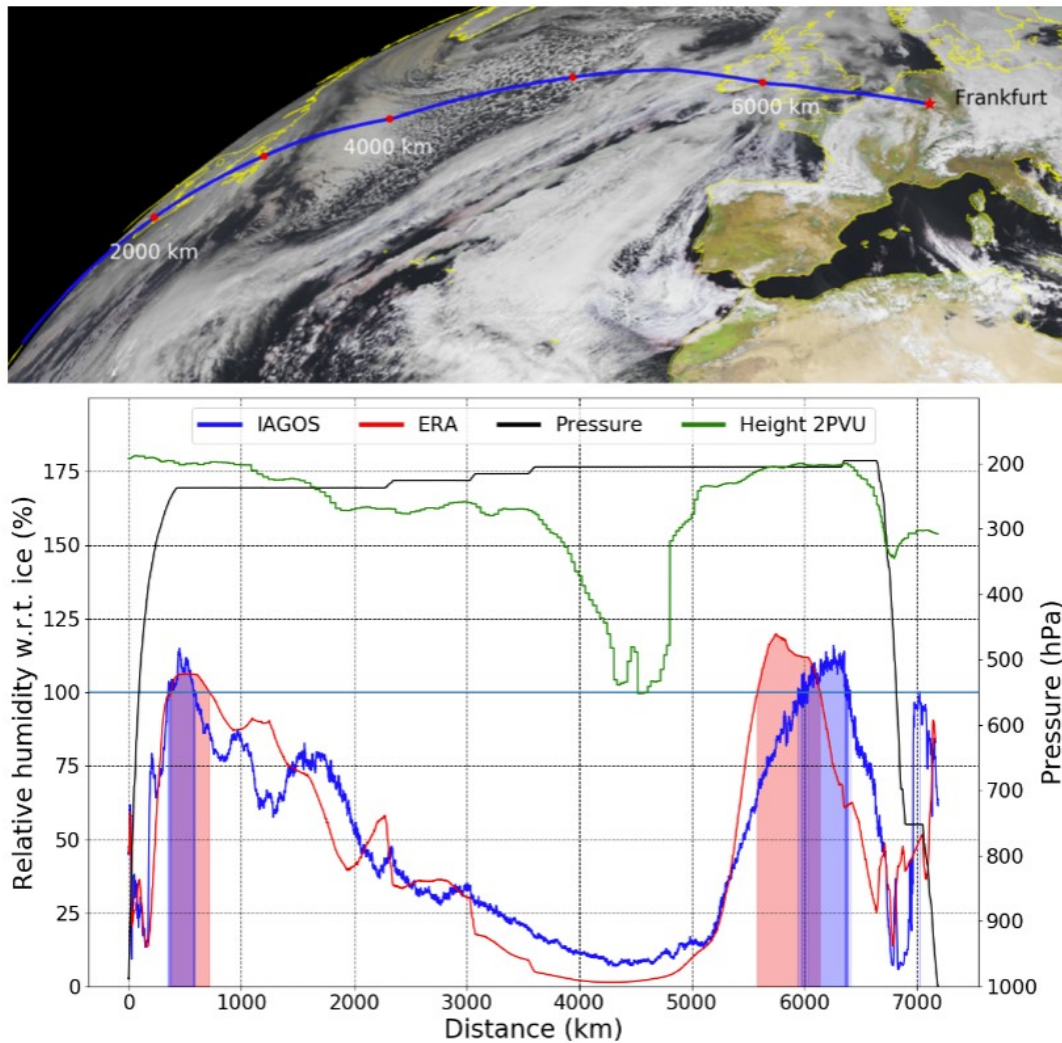
Figure 8. Example of typical flight from Atlanta (USA) to Frankfurt (Germany) on March 7th, 2009. The upper part shows the synoptic situation over the North Atlantic on that day including the flight path. For better orientation red dots are placed every 1000 km. In the lower part RH i is shown over the distance of the flight for IAGOS (blue) and ERA (red). Shaded areas denote ice supersaturation. The pressure level of the aircraft is shown in black and the height in hPa of the dynamical tropopause (2PVU) is shown in green. Satellite image: copyright 2009 EUMETSAT.
