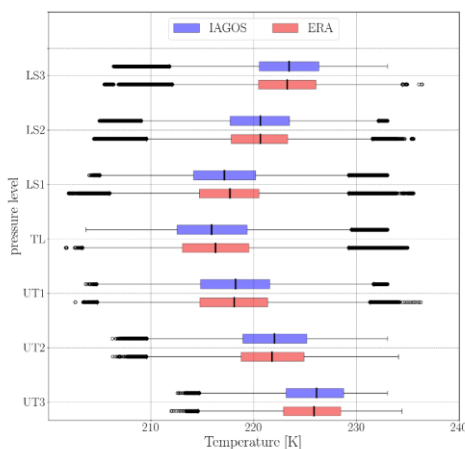
Figure 2. Vertical profile of temperature [K] for IAGOS (left, blue) and ERA (right, red).
