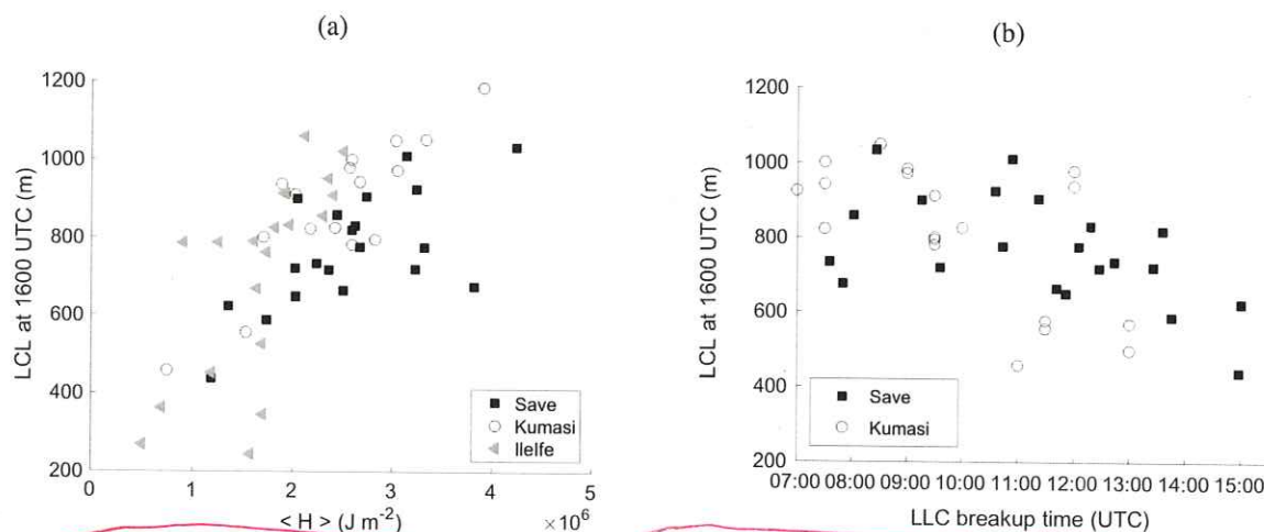
Figure 9. LCL at 1600 UTC against \langle H \rangle at the three sites (a). LCL at 1600 UTC against LLC breakup time at Savè and Kumasi (b). The LLC breakup time can not be estimated in Ile-Ife.
