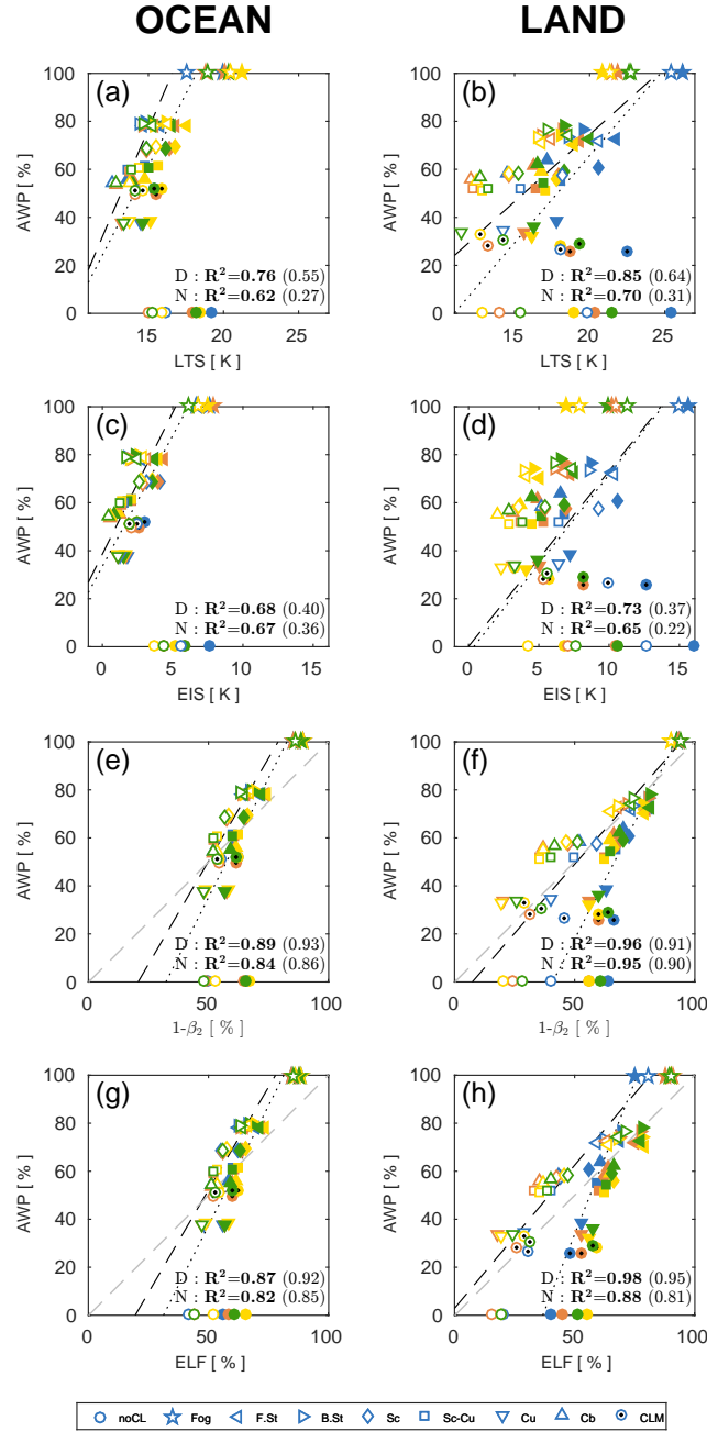
Figure 6. Scatter plots of Fig. 5 over the (left) ocean and (right) land during the daytime (open symbols) and nighttime (filled symbols), respectively. Also plotted are the linear regression lines and squared correlation coefficients ( R^2 ) during the daytime (D, dashed) and nighttime (N, dotted), respectively. The bold R^2 are the values when CLM and noCL are excluded in the regression analysis, and the R^2 in the parenthesis are the values when Fog is additionally excluded. The seasons were marked with the same colors as Fig. 5. The dashed gray lines in the last four plots denote AWP=ELF .
