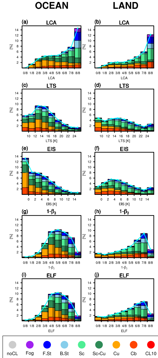
Figure 8. Same as Fig. 7 but for AMT of individual CL in each bin. The cyan lines are identical to those shown in Fig. 7. The sum of all CLs' AMT integrated over the entire bins is the global annual-mean LCA, which is identical regardless of the proxies used for the composite.
