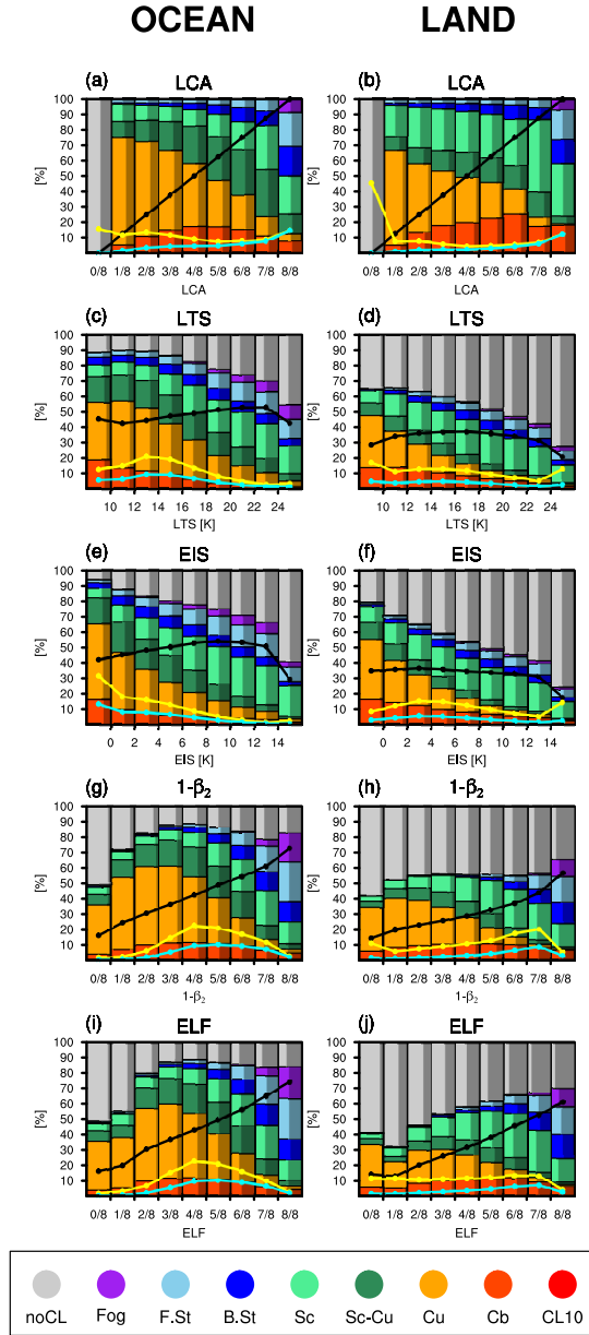
Figure 7. Stacked percentage plots for the FQs of individual CLs in the bins of various proxies, (a),(b) LCA (i.e., a perfect proxy for LCA), (c),(d) LTS, (e),(f) EIS, (g),(h) 1-\beta_2 , and (i),(j) ELF over the (left) ocean and (right) land, respectively. AWP of all CLs in each bin is denoted by the black line. The observation number FQ of individual bin (the ratio of the observation number in each bin to the total observation number of entire bins) is denoted by the yellow line. LCA in each bin is denoted by the cyan line, which is the product of the black and yellow lines. The sum of the yellow line integrated over the entire bins is 100%. The sum of the cyan line integrated over the entire bins is the global-annual mean LCA. The bright and dark colors in each bar denote the fractions during the daytime and nighttime, respectively.
