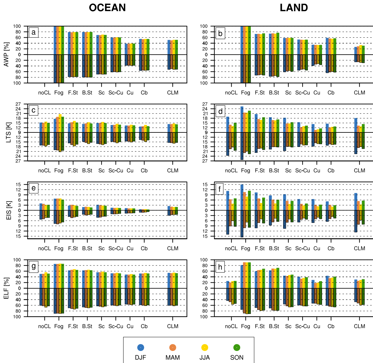
Figure 5. Seasonal climatologies of the (1st row) AWP, (2nd) LTS, (3rd) EIS, and (4th) ELF averaged over the (left) ocean and (right) land for each season (DJF, MAM, JJA, SON denoted by different colors) during the daytime (09 am - 09 pm, upward bars with bright colors) and nighttime (09 pm - 09 am, downward bars with dark colors), respectively, when a specific CL was reported. In each plot, CLM denotes the climatology for all CLs.
