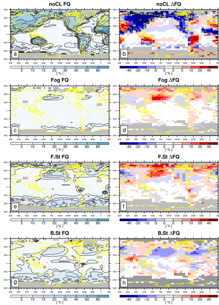
Figure 1. (First column) The annual mean climatological CL frequency (FQ) and (second column) the differences of climatological CL FQ between JJA and DJF [ \Delta FQ = FQ(JJA) - FQ(DJF) ] for (a)(b) noCL, (c)(d) Fog, (e)(f) F.St, and (g)(h) B.St. In the first column, the grid boxes with total observation number less than 100 are shaded with a gray color. In the second column, statistically insignificant \Delta FQ at the 99.9 % confidence level from the two-sided Student t-test assuming independent samples are denoted by white color, and the grid boxes with the observation number less than 100 during either JJA or DJF are shaded with a gray color.
