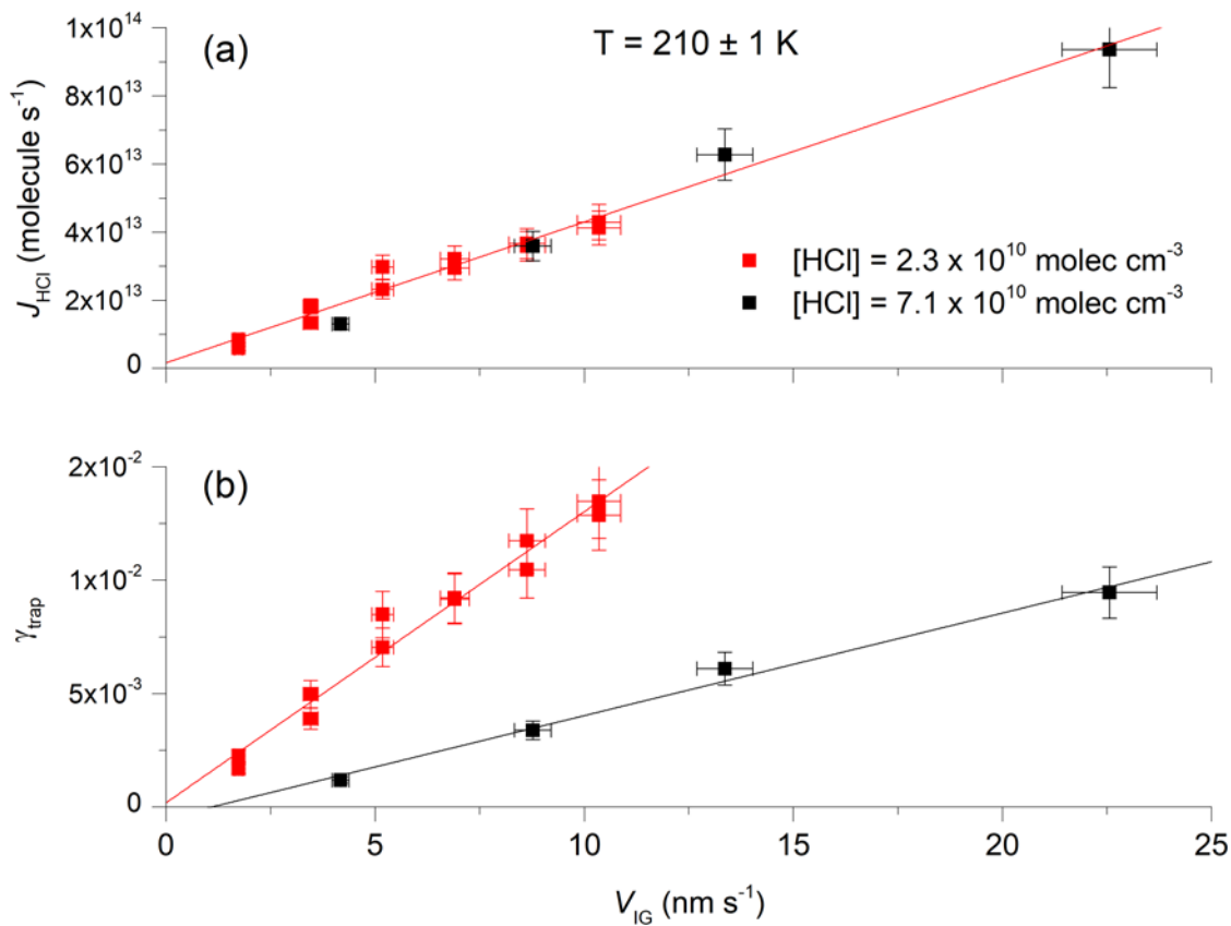
Figure 3: The trapping coefficient ( \gamma_{trap} ) as a function of ice growth velocity at 210 K using two different concentrations of HCl. The solid, straight lines are least-squares fits to the data. The error bars represent total uncertainty in \gamma_{trap} and the ice growth velocity.
