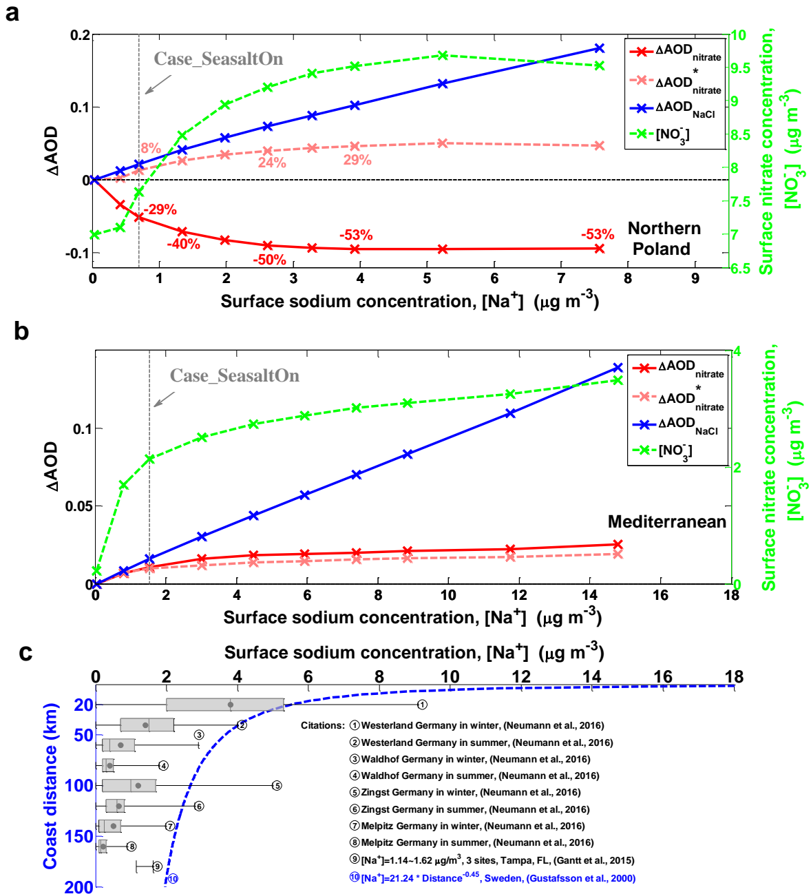
Fig. 6. Sensitivity of aerosol optical depth ( \Delta AOD ) as a function of sodium mass concentration ( [Na^+] ). Differences between the ‘Case_SeasaltOff’ and sensitivity cases (sea-salt emission with different scaling factors) for different aerosol components, i.e., nitrate ( \Delta AOD_{nitrate} ) and sea-salt ( \Delta AOD_{NaCl} ): \Delta AOD (sensitivity case – ‘Case_SeasaltOff’) versus [Na^+] over northern Poland (a) and Mediterranean regions (b), respectively. The model results shown here are averages over a sea-salt event during daytime (07:00-16:00 LT) on 19 September 2013. The results of surface [NO_3^-] are indicated by the green dashed line. Here, the ‘Case_SeasaltOff’ is the reference case and the ‘Case_SeasaltOn’ is marked. Note: \Delta AOD_{nitrate}^* (pink dashed line) indicates the \Delta AOD of nitrate calculated by re-allocating nitrate mass into different size bins according to the normalized nitrate particle mass size distribution simulated in ‘Case_SeasaltOff’ (i.e., without ‘re-distribution effect’). c, The measured [Na^+] at different sites over Sweden as a function of coast distance, and in Germany (marked in Fig. 3) and US. The box-whisker plots of the references ①-⑧ indicate the median, mean (black dot), 25% percentile, 75% percentile, maximum and minimum. The error bar of the reference ⑨ indicates the range. The blue dashed line of the reference ⑩ indicates the statistically empirical function of [Na^+] with the distance from coast, based on the network measurements of 16 sites in Sweden.
