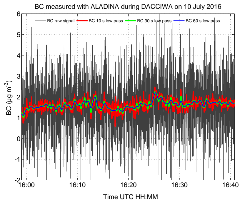
Figure 3. The BC mass concentration measured during one flight between 15:58 and 16:42 UTC on 10 July 2016. The raw signal of BC (grey line) was phase shift free low pass filtered after post-processing with 10 s (red line), 30 s (green line) and 60 s (blue line).
