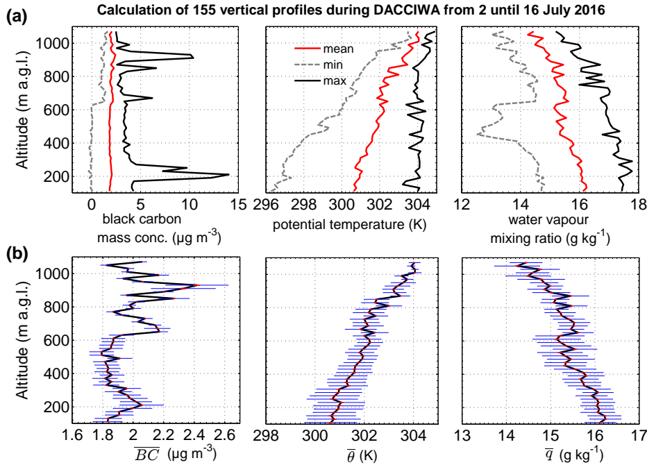
Figure 5. Summary of 155 vertical profiles from 100 to 1100 m a.g.l. measured with ALADINA during the field experiment of DACCIWA lasting from 2 until 16 on 2–16 July 2016. From left to right: Vertical profiles of black carbon mass concentration (BC) measured with the aethalometer and 10 s low pass filtering, potential temperature \theta and water vapour mixing ratio q . The red line represents the mean value, the grey dashed lines stands for the total minimum and the black solid line is the total maximum of all vertical profiles, averaged in 20 m altitude intervals. At the bottom: The mean values of BC ( \overline{BC} ), \theta ( \overline{\theta} ) and q ( \overline{q} ) in the 20 m steps, and the corresponding standard deviation for each height interval.
