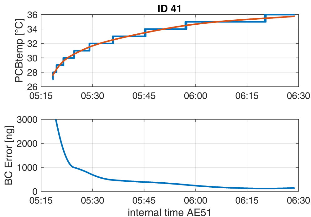
Figure 2. The impact of the temperature changes on the BC mass concentration. The figure shows the internal temperature (PCBtemp) of the aethalometer AE51 during the measurement flight on 14 July 2016 from 05:16 until 06:30 UTC on 14 July 2016 (top). The bit noise was smoothed for the time interval (red line). The figure at the bottom represents the calculated error of the black carbon mass concentration.
