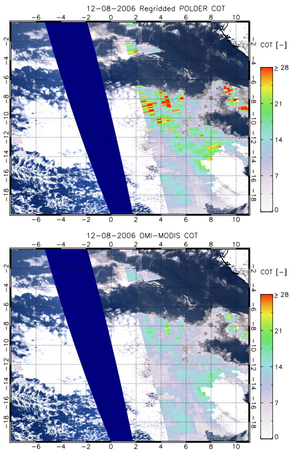
Figure 6. Cloud optical thickness (COT) overplotted on a MODIS RGB image on 12 August 2006 for POLDER at 0.87 \mu\text{m} regridded to OMI grid (upper panel) and OMI-MODIS at 1.2 \mu\text{m} (lower panel).
