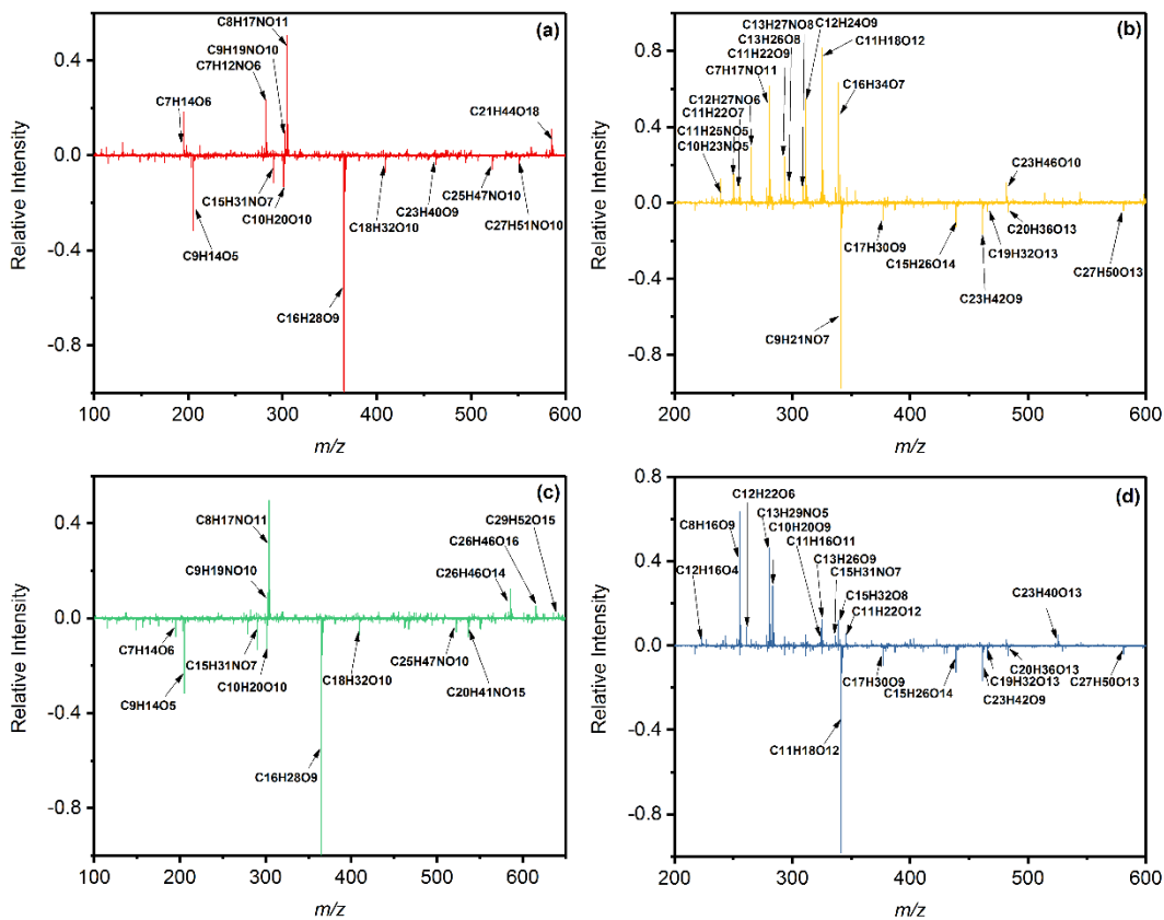
5 Figure 4. Results of mass spectra difference of toluene SOA under the DS condition minus the WS condition in (a) positive and (b) negative mode, and of the W condition minus the WS condition in (c) positive and (d) negative mode. Y axis is the subtraction of relative intensity (indicated by the peak intensity relative to the strongest peak intensity) between condition DS or W and WS.
