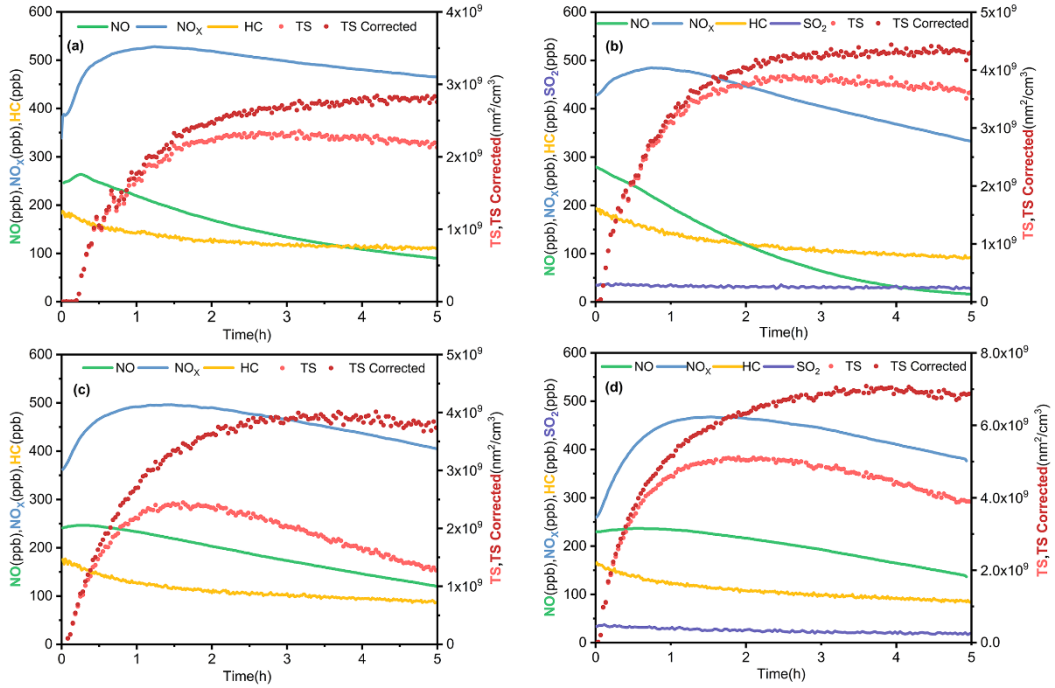
Figure 1. Reaction profiles of photooxidation of toluene under four different conditions: (a) D1 (dry condition), (b) DS1 (dry condition with SO 2 ), (c) W1 (wet condition) and (d) WS1 (wet condition with SO 2 ); see Table 1 for details. The concentrations of gas species are shown on the left axis, while the concentrations of particles are shown on the right axis.
