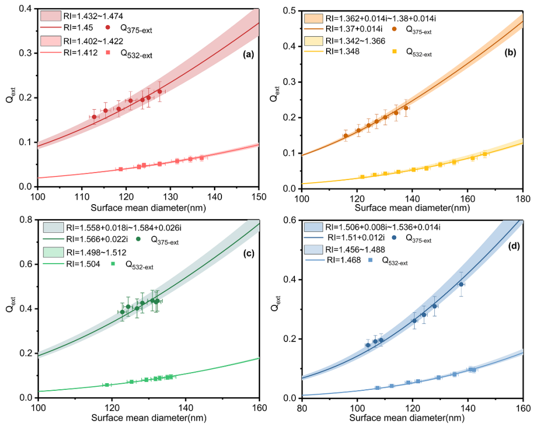
Figure 2. Dependence of the extinction efficiencies of the SOA on the surface mean diameter under four different conditions of (a) D1, (b) DS1, (c) W1 and (d) WS1. The lines are results retrieved from the average RI, while the shadows are ranges of the retrieved RI.
