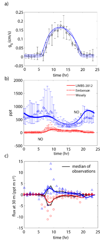
Figure 4: Comparison of model results to (a) hourly averaged observed stomatal conductances, (b) NO and NO 2 mixing ratios at 30 m, and (c) median (black lines) and hourly-averaged NO and NO 2 vertical fluxes at 30 m observed during UMBS-2012 for August 8, 2012. In all panels solid lines, dotted lines, and dashed lines, represent results from our model with stomatal conductances parameterized using observed conductances, the Wesely model, and the Emberson model, respectively. Blue triangles and red circles represent NO 2 and NO observations, respectively. Error bars represent the interquartile range of data.
