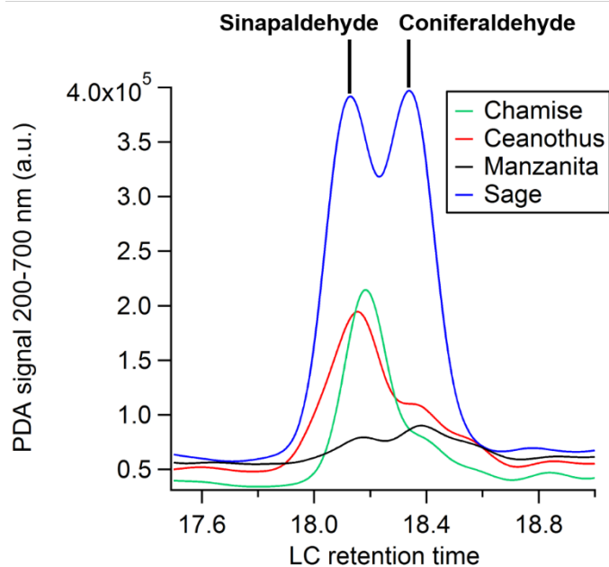
Figure 2. Lignin pyrolysis products sinapaldehyde ( \text{C}_{11}\text{H}_{12}\text{O}_4 ) and coniferaldehyde ( \text{C}_{10}\text{H}_{10}\text{O}_3 ) elute at slightly different retention times, at roughly 18.1 and 18.4 min, respectively.
