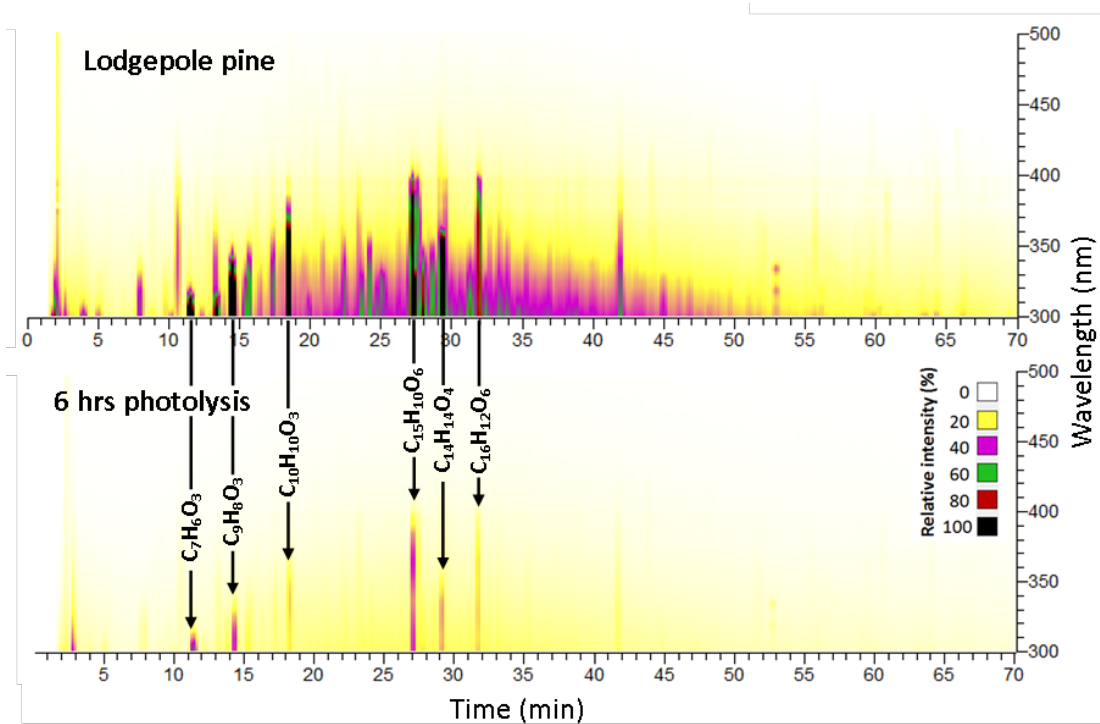
Figure 3. BrC chromophores present in the BBOA sample before (top panel) and after (bottom panel) 300 nm irradiation for a conifer fuel, lodgepole pine.
