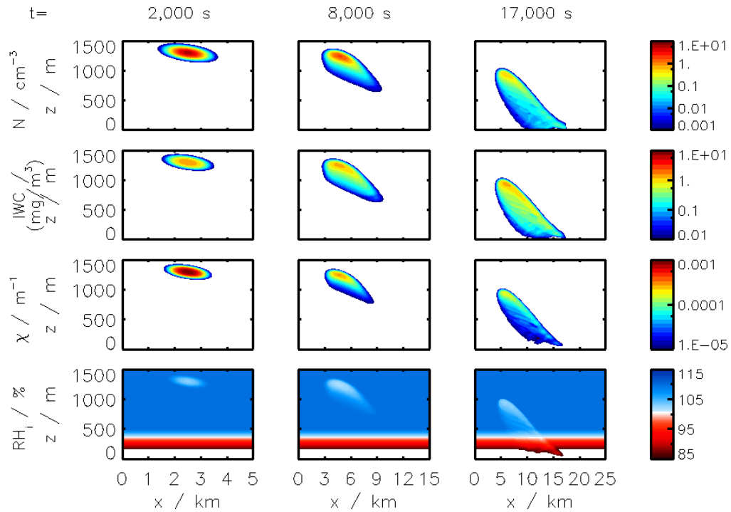
Figure D2. Ice crystal concentration N , ice mass concentration \text{IWC} , extinction \chi and relative humidity \text{RH}_i for the same conditions as described in Unterstrasser and Gierens (2010a). The flight level is at a vertical distance of 1,300 m.
