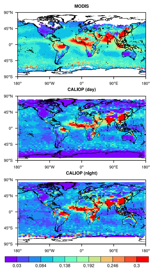
Figure 12. Spatial distributions of the monthly mean MODIS Aqua AOTs at 550 nm, day-time CALIOP and night-time CALIOP AOTs at 532 nm in November from 2006 to 2016.
