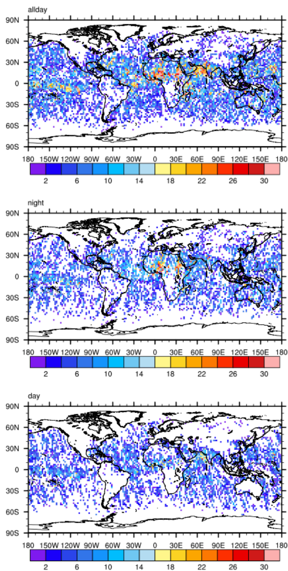
Figure S3. Total number of available CALIOP hourly aerosol extinction coefficients during November 2016 throughout the day, in the night-time, and in the day-time.
