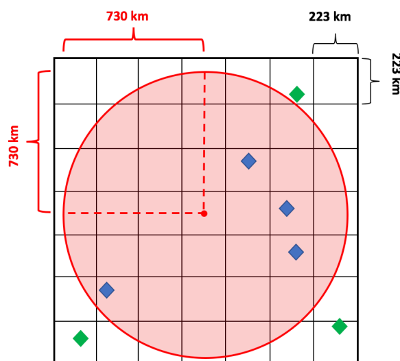
Figure A1. A schematic showing the horizontal observation localization. The observations located within the red circle as the blue diamonds are used for assimilation. The observations located out of the red circle as the green diamonds are not used for assimilation.
