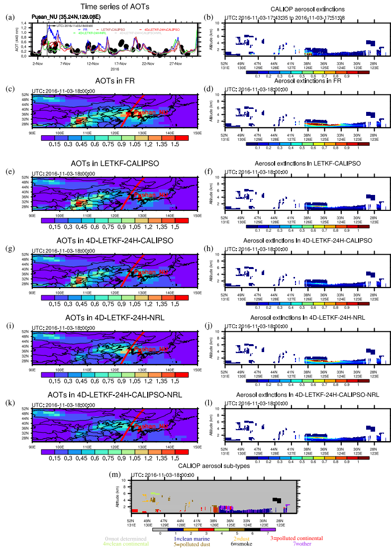
Figure 10. (a) Hourly time series of the AOTs at 440 nm for the FR, LETKF-CALIPSO, 4D-LETKF-24H-CALIPSO, 4D-LETKF-24H-NRL, and 4D-LETKF-24H-CALIPSO-NRL experiments and the observed AOTs from Aerosol Robotic Network (AERONET) over Pushan_NU site during November 2016. The root-mean-square error (RMSE) and correlation coefficient (CORR) between the simulated and the observed AOTs are also shown. The spatial distributions of the simulated AOTs at 440 nm at 18:00:00 (UTC) 3 November 2016 in the FR (c), LETKF-CALIPSO (e), 4D-LETKF-24H-CALIPSO (g), 4D-LETKF-24H-NRL (i), and 4D-LETKF-24H-CALIPSO-NRL (k) experiments. The red triangle indicates the location of Pushan_NU site. The red curve indicates one CALIPSO orbit path near the Pushan_NU site on 3 November 2016. The CALIOP observed aerosol extinction coefficients at 532 nm [ \text{km}^{-1} ] (b) and the simulated ones at 550 nm in the FR (d), LETKF-CALIPSO (f), 4D-LETKF-24H-CALIPSO (h), 4D-LETKF-24H-NRL (j), and 4D-LETKF-24H-CALIPSO-NRL (l) experiments over that CALIPSO orbit path. (m) CALIPSO derived vertical aerosol sub-types.
