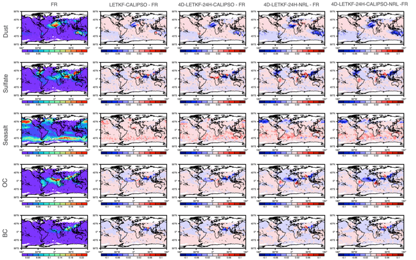
Figure S2. Spatial distributions of the monthly mean AOTs at 550 nm in the FR experiment (sampled to the NRL MODIS observations) and the mean differences of the AOTs in the LETKF-CALIPSO, 4D-LETKF-24H-CALIPSO, 4D-LETKF-24H-NRL, and 4D-LETKF-24H-CALIPSO-NRL experiments minus those in the FR experiment for each individual aerosol component (i.e., dust, sulfate, sea salt, organic carbon [OC], and black carbon [BC]) during November 2016.
