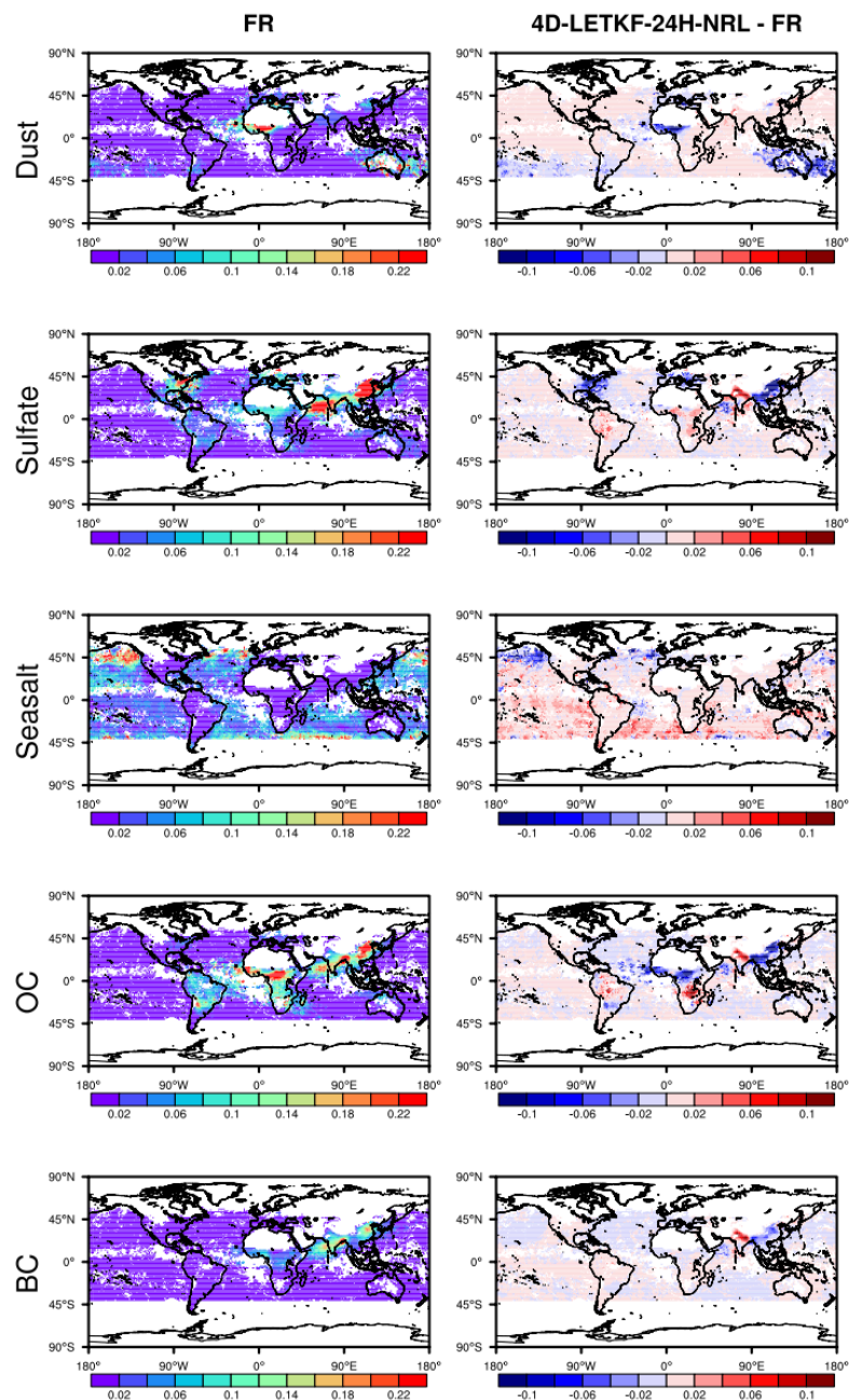
Figure S1. Spatial distributions of the monthly mean AOTs at 550 nm in the FR experiment (sampled to the MODIS Aqua observations) and the mean differences of the AOTs in the 4D-LETKF-24H-NRL experiment minus those in the FR experiment for each individual aerosol component (i.e., dust, sulfate, sea salt, organic carbon [OC], and black carbon [BC]) during November 2016.
