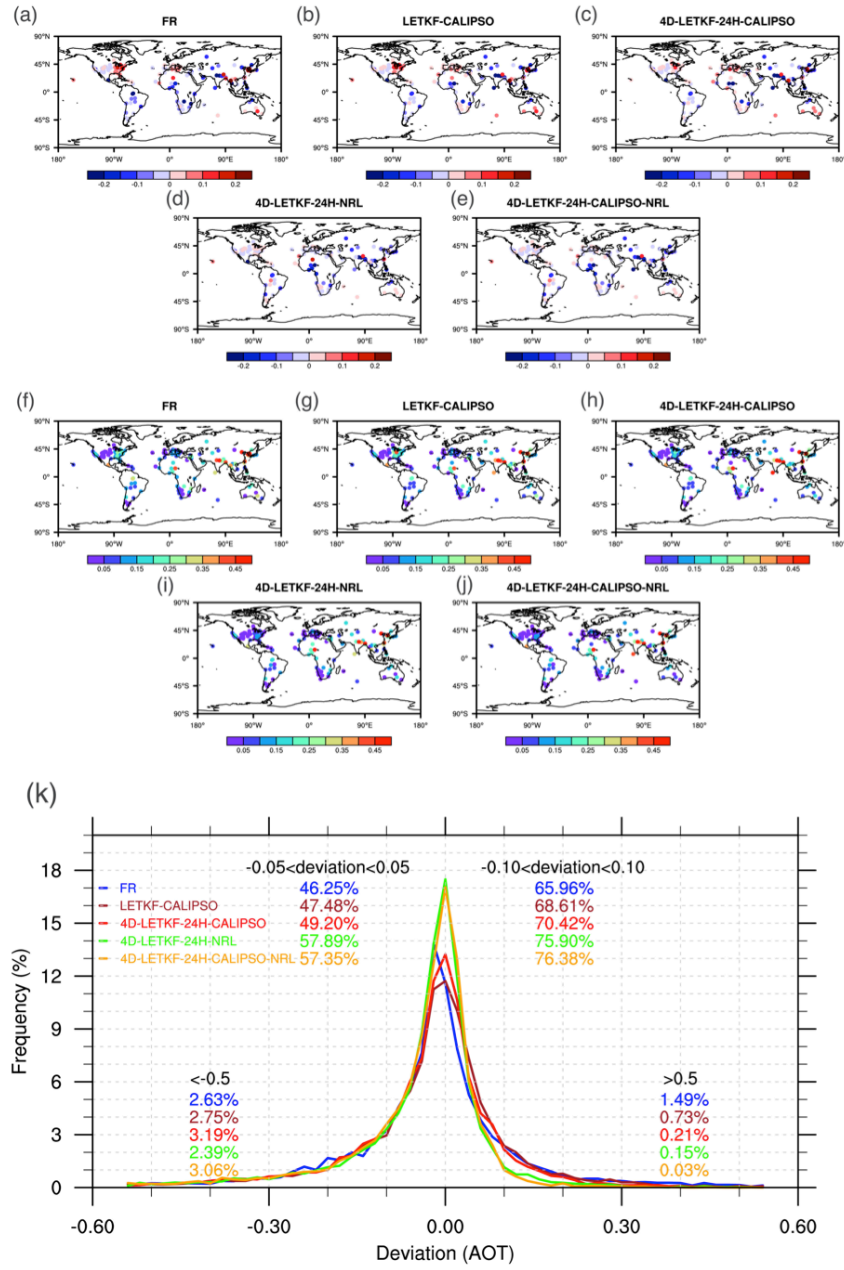
Figure 9. Same as Figure 8 but for the simulated AOTs at 440 nm against the AERosol RObotic NETwork (AERONET)-retrieved ones.
